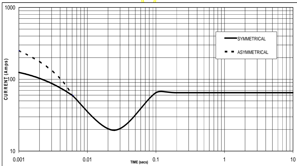
Sustained Short Circuit = 65 Amps
