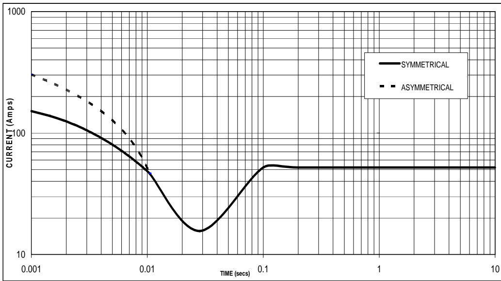
Sustained Short Circuit = 52 Amps
