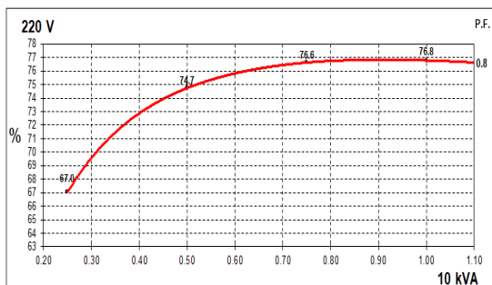
50Hz Curves
