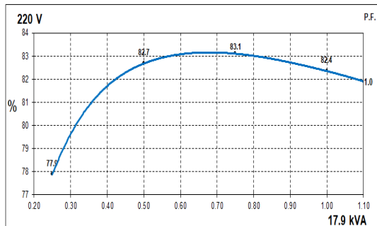
50Hz Curves
