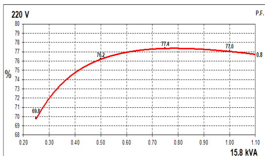
50Hz Curves
