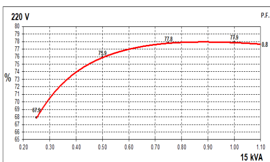
60Hz Curves
