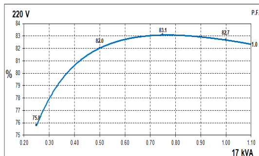
60Hz Curves
