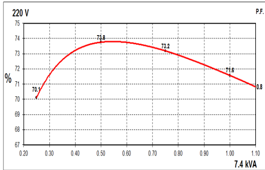
50Hz Curves
