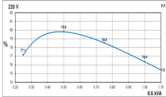
60Hz Curves
