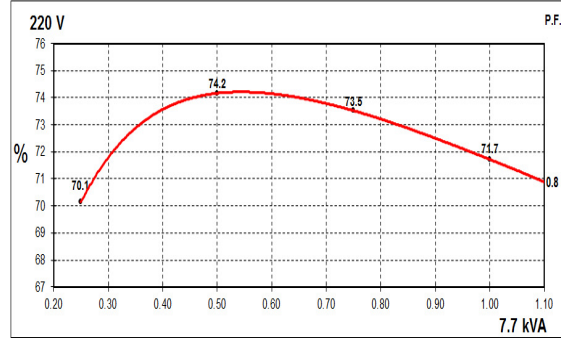
60Hz Curves
