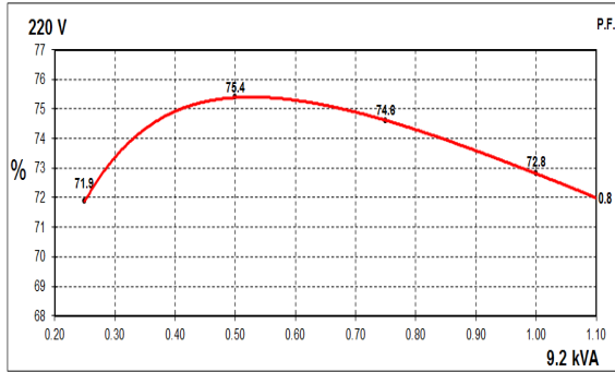
60Hz Curves
