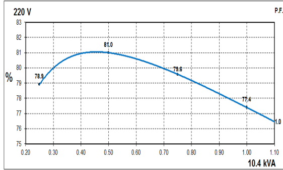
60Hz Curves
