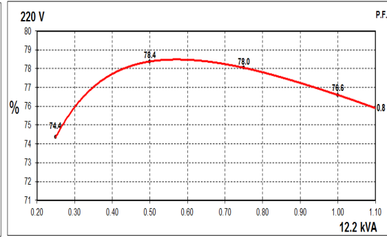
60Hz Curves
