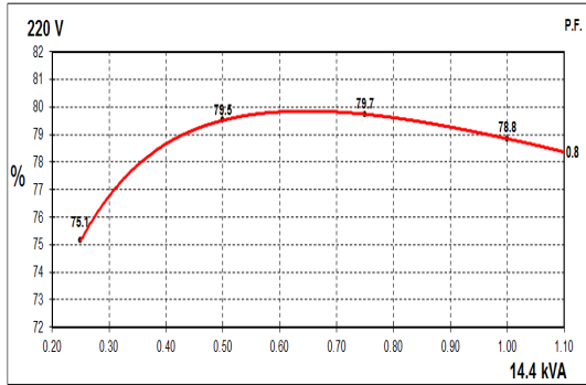
50Hz Curves
