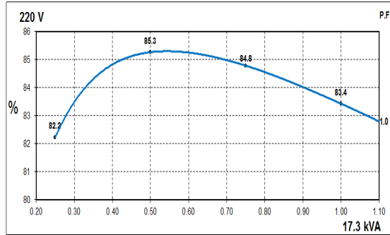
60Hz Curves
