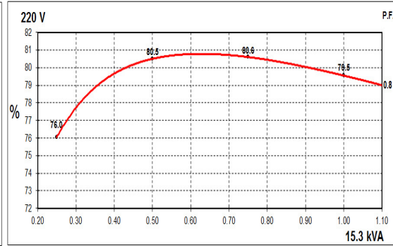
60Hz Curves
