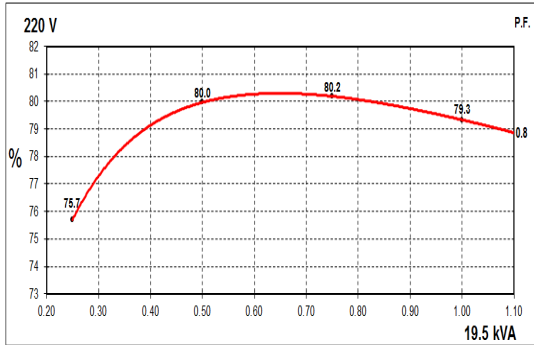
50Hz Curves
