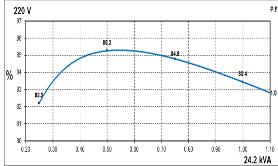
60Hz Curves
