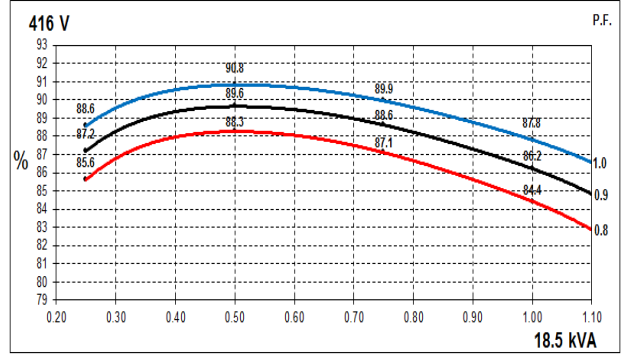
60Hz Curves
