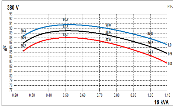
50Hz Curves
