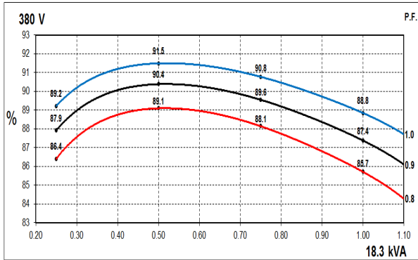
50Hz Curves
