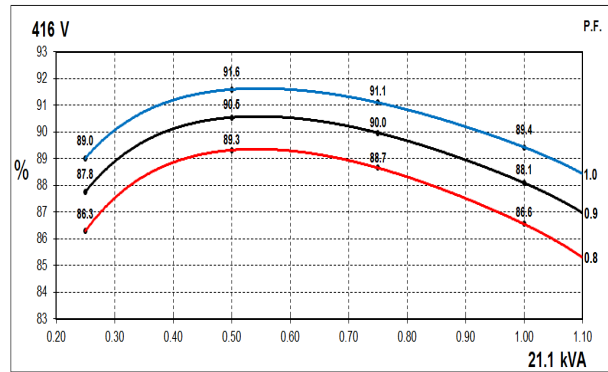
60Hz Curves
