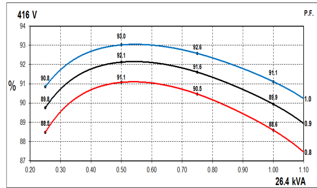
60Hz Curves
