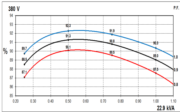
50Hz Curves
