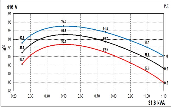
60Hz Curves
