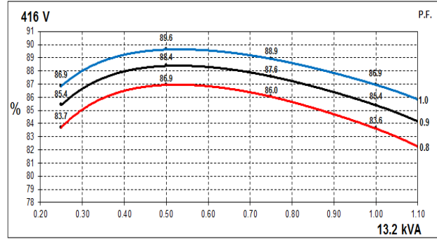
60Hz Curves
