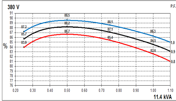
50Hz Curves
