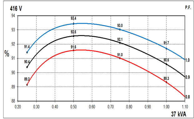
60Hz Curves
