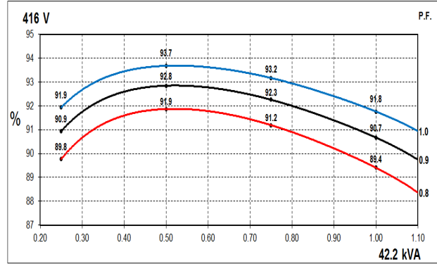
60Hz Curves
