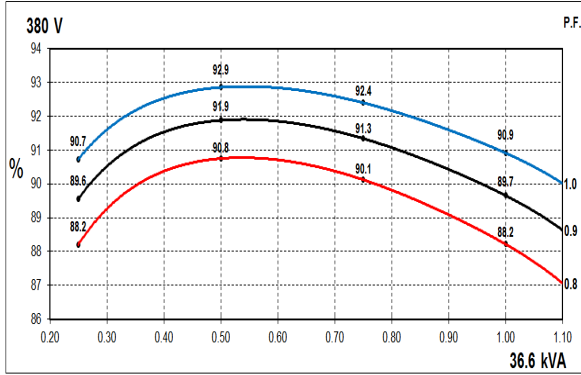
50Hz Curves
