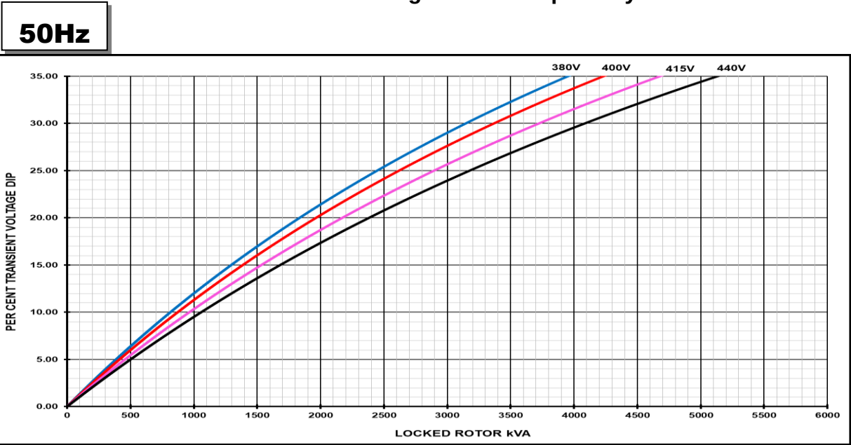
Locked Rotor Motor Starting Curves - Separately Excited
