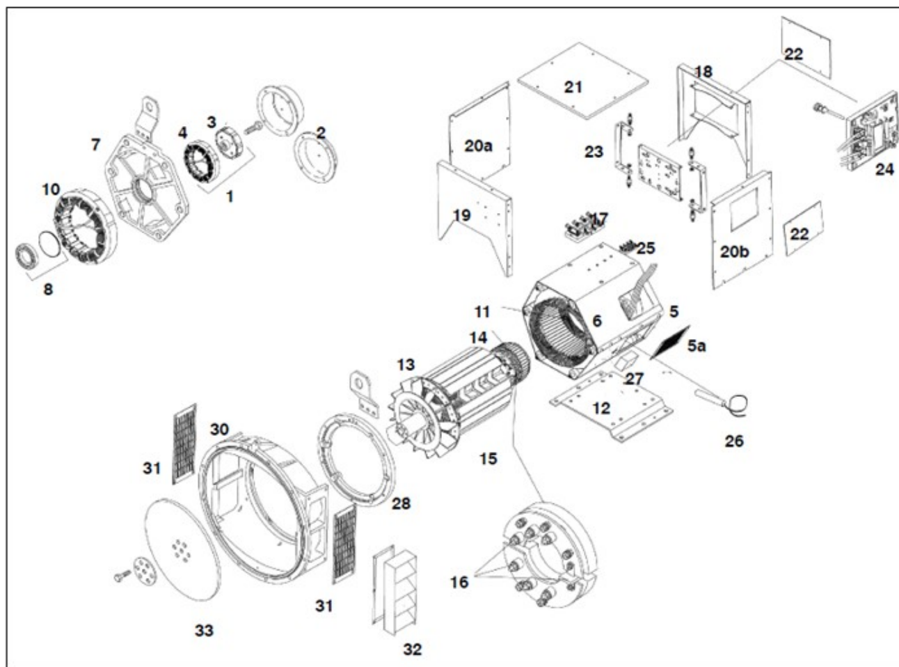
FIGURE 14. UCI224 - ONE BEARING ALTERNATOR PARTS DRAWING
