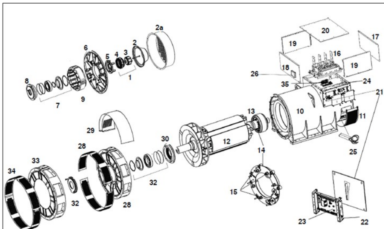
FIGURE 34. P7 (A-G) TWO BEARING ALTERNATOR PARTS DRAWING
