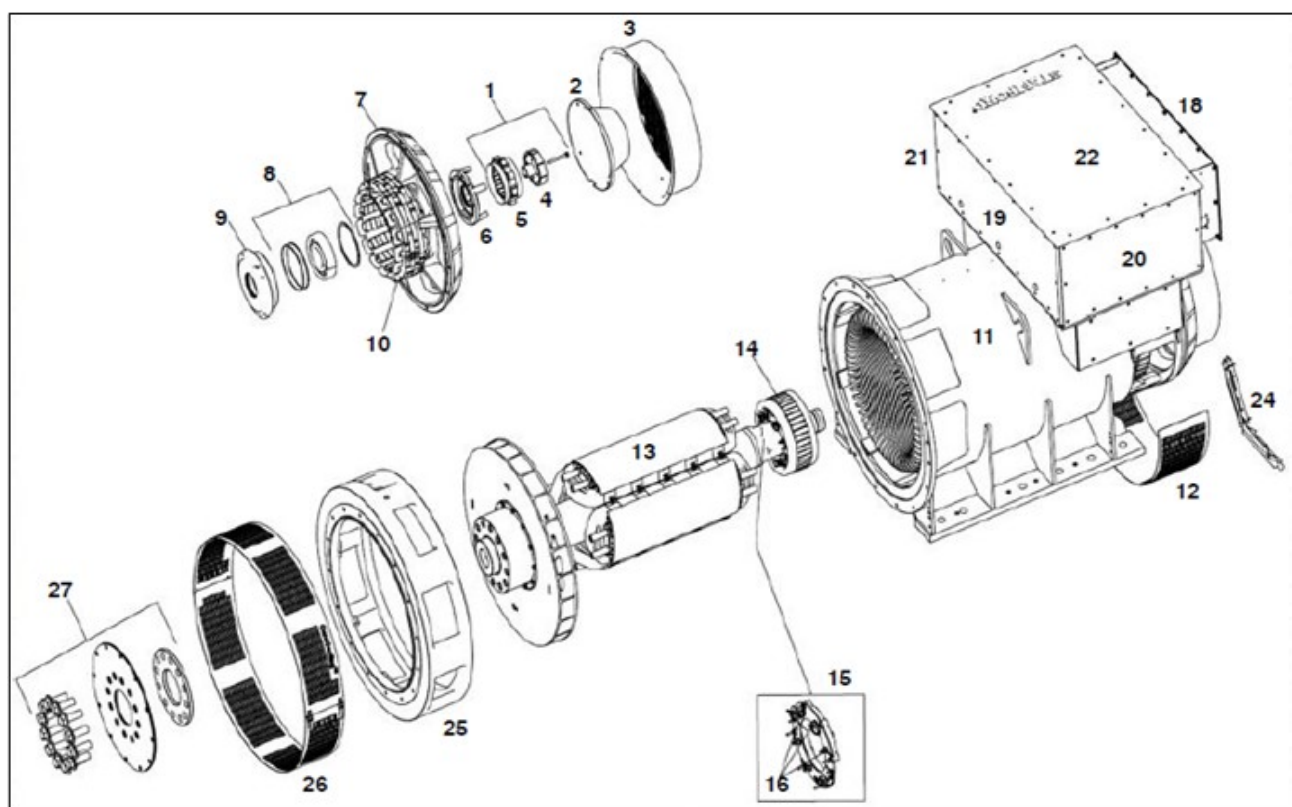
FIGURE 38. S7 HV ONE BEARING ALTERNATOR PARTS DRAWING
