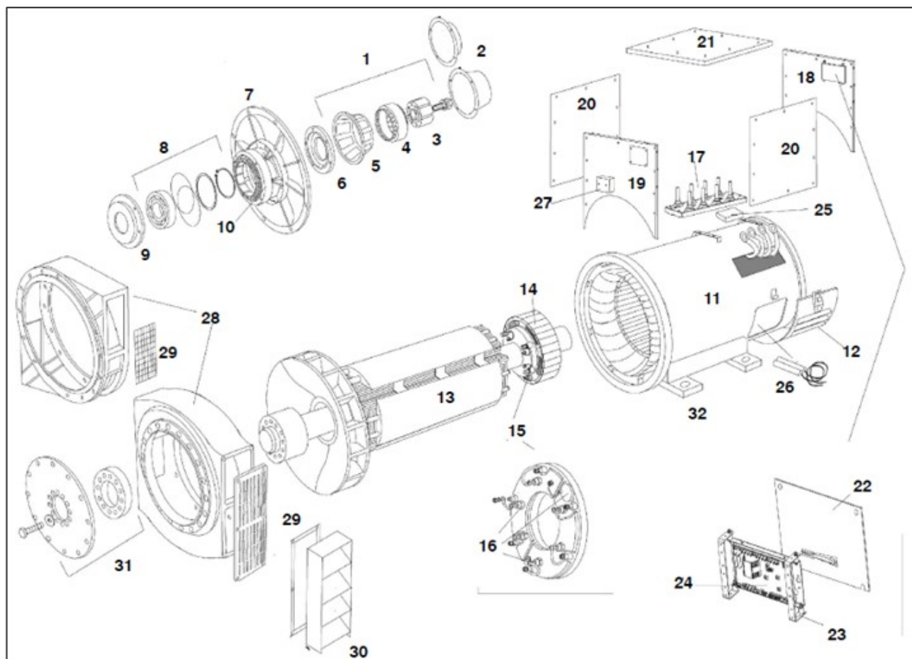
FIGURE 18. HC434 (C-F) ONE BEARING ALTERNATOR PARTS DRAWING
