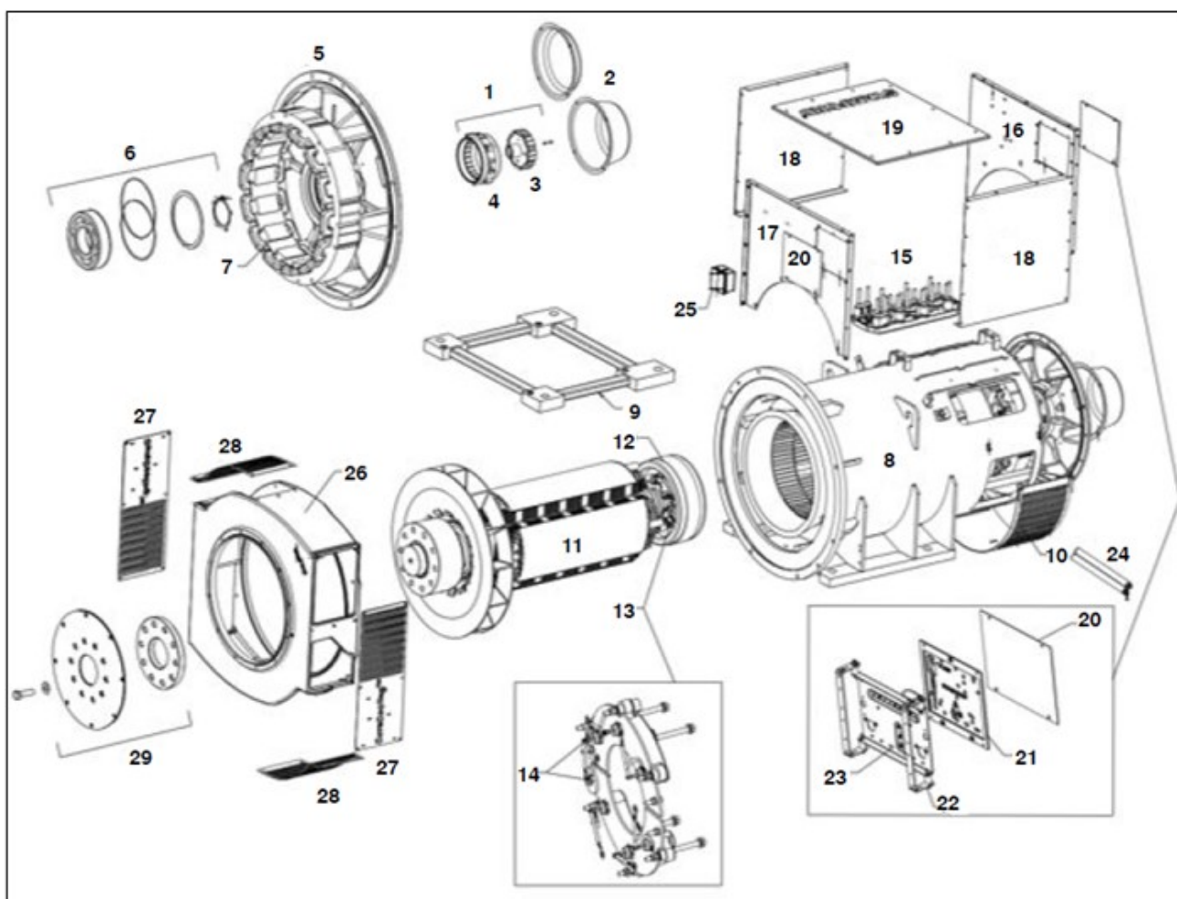
FIGURE 26. S5 (G-H) ONE BEARING (DEDICATED) ALTERNATOR PARTS DRAWING
