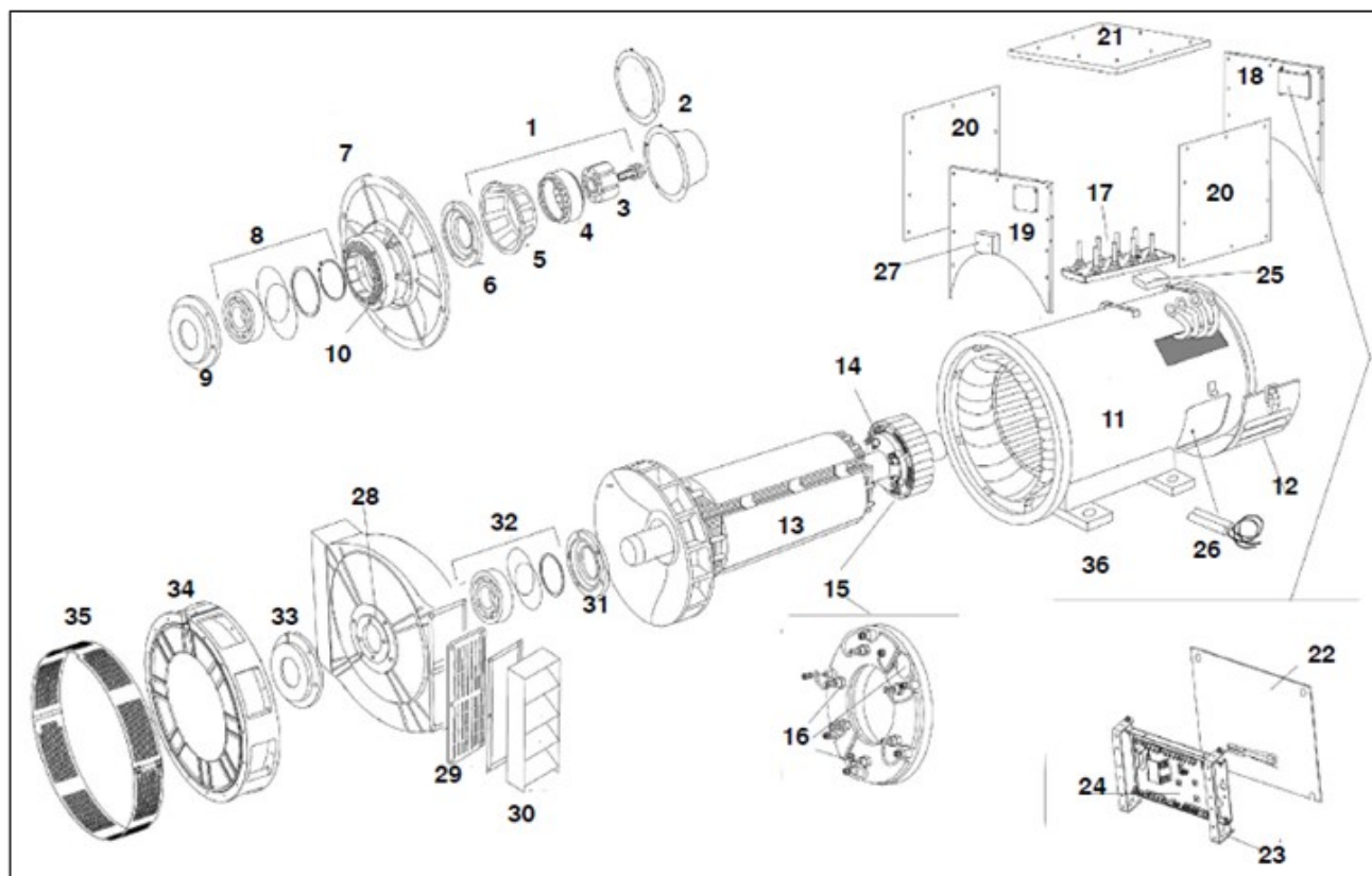
FIGURE 19. HC434 (C-F) TWO BEARING ALTERNATOR PARTS DRAWING
