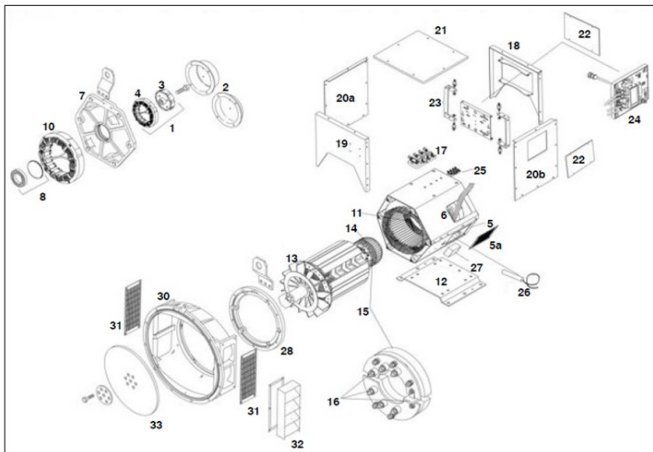
FIGURE 13. UCD27 - ONE BEARING ALTERNATOR PARTS DRAWING
