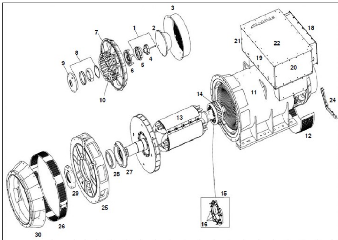
FIGURE 39. S7 HV TWO BEARING ALTERNATOR PARTS DRAWING
