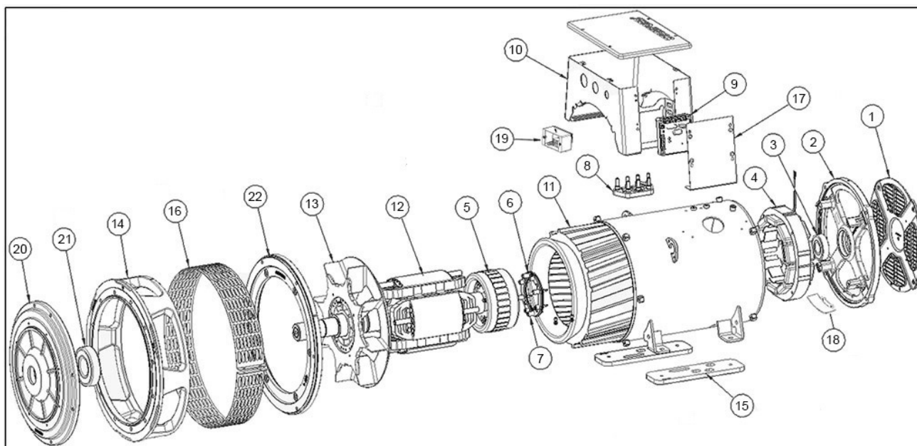
FIGURE 9. S0L1 - TWO BEARING ALTERNATOR PARTS DRAWING
