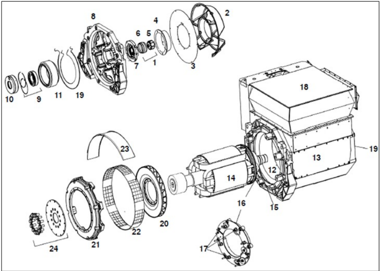
FIGURE 43. P80 ONE BEARING PARTS DRAWING
