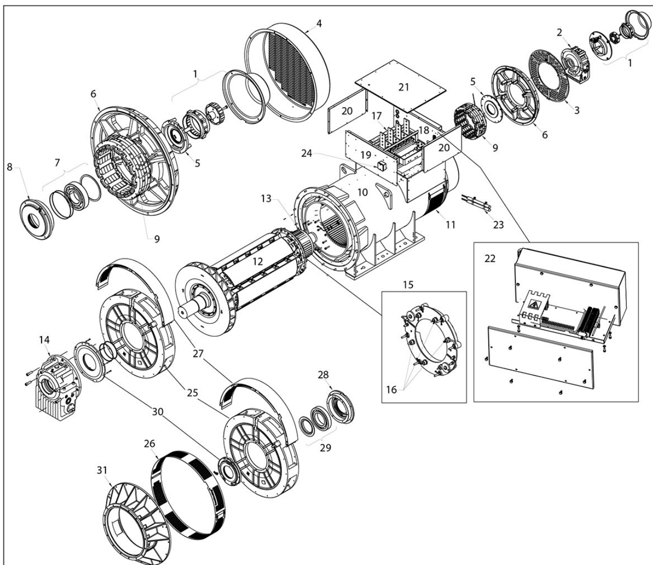
FIGURE 41. A7 LV TWO BEARING ALTERNATOR PARTS DRAWING
