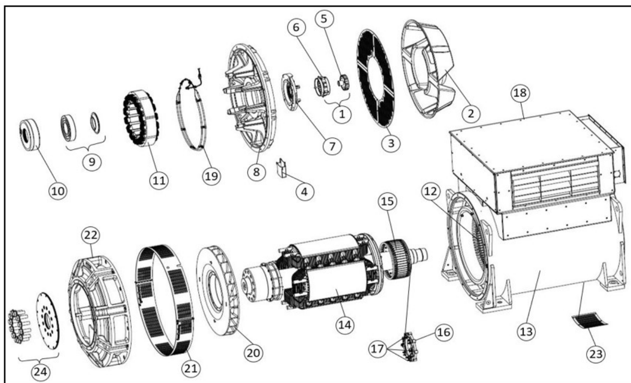
FIGURE 45. S9 LV ONE BEARING ALTERNATOR PARTS DRAWING
