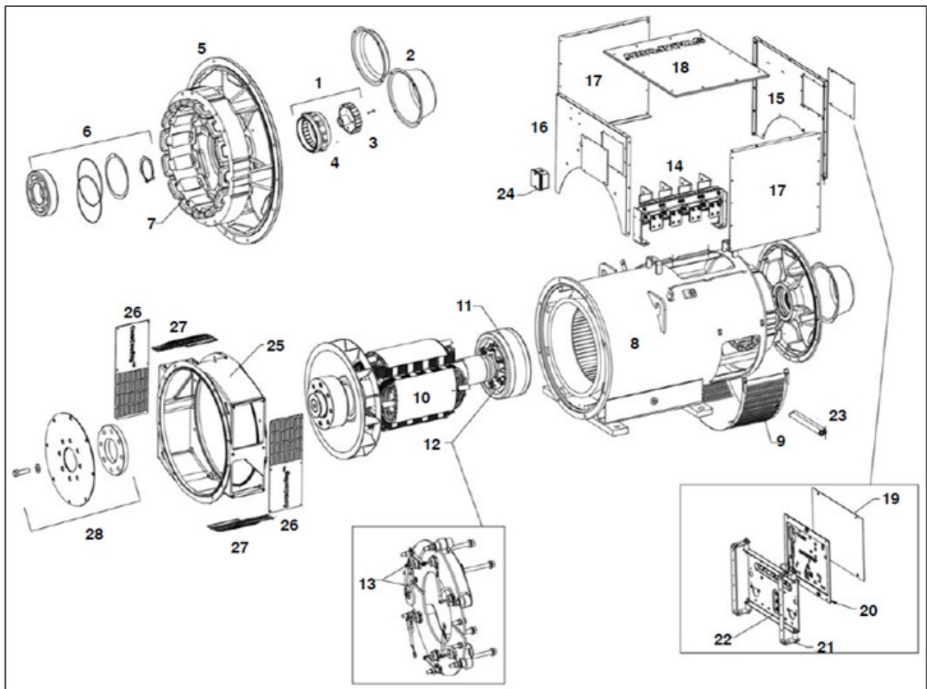
FIGURE 25. S5 (C-F) ONE BEARING (DEDICATED) ALTERNATOR PARTS DRAWING
