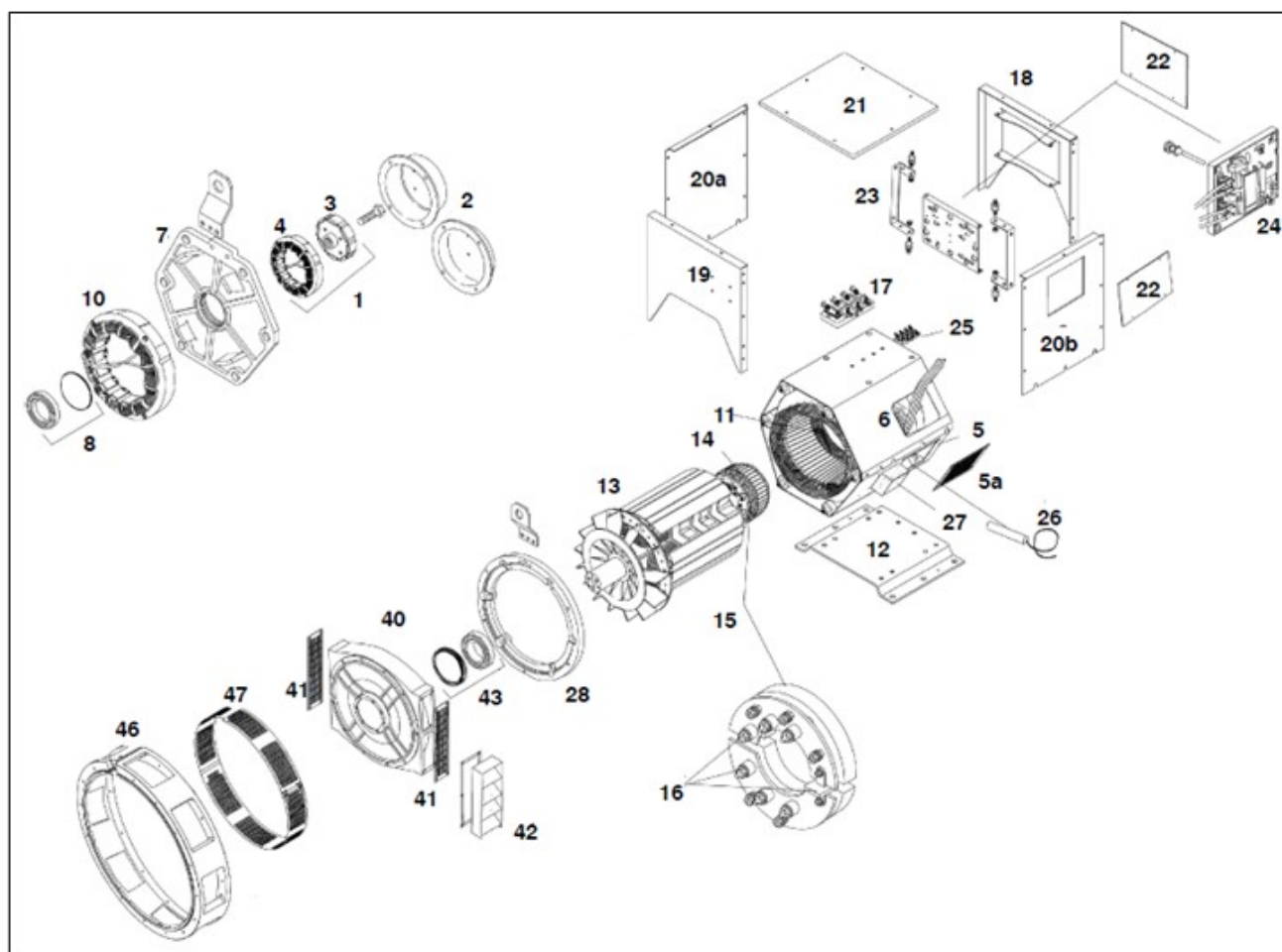
FIGURE 17. UCI274 (C-H) TWO BEARING (4 POLE) ALTERNATOR PARTS DRAWING
