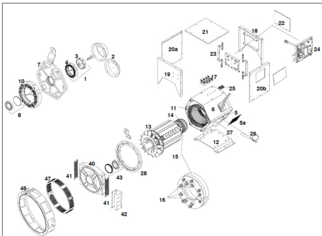
FIGURE 15. UCI224 (C-G) TWO BEARING 4 POLE PARTS DRAWING
