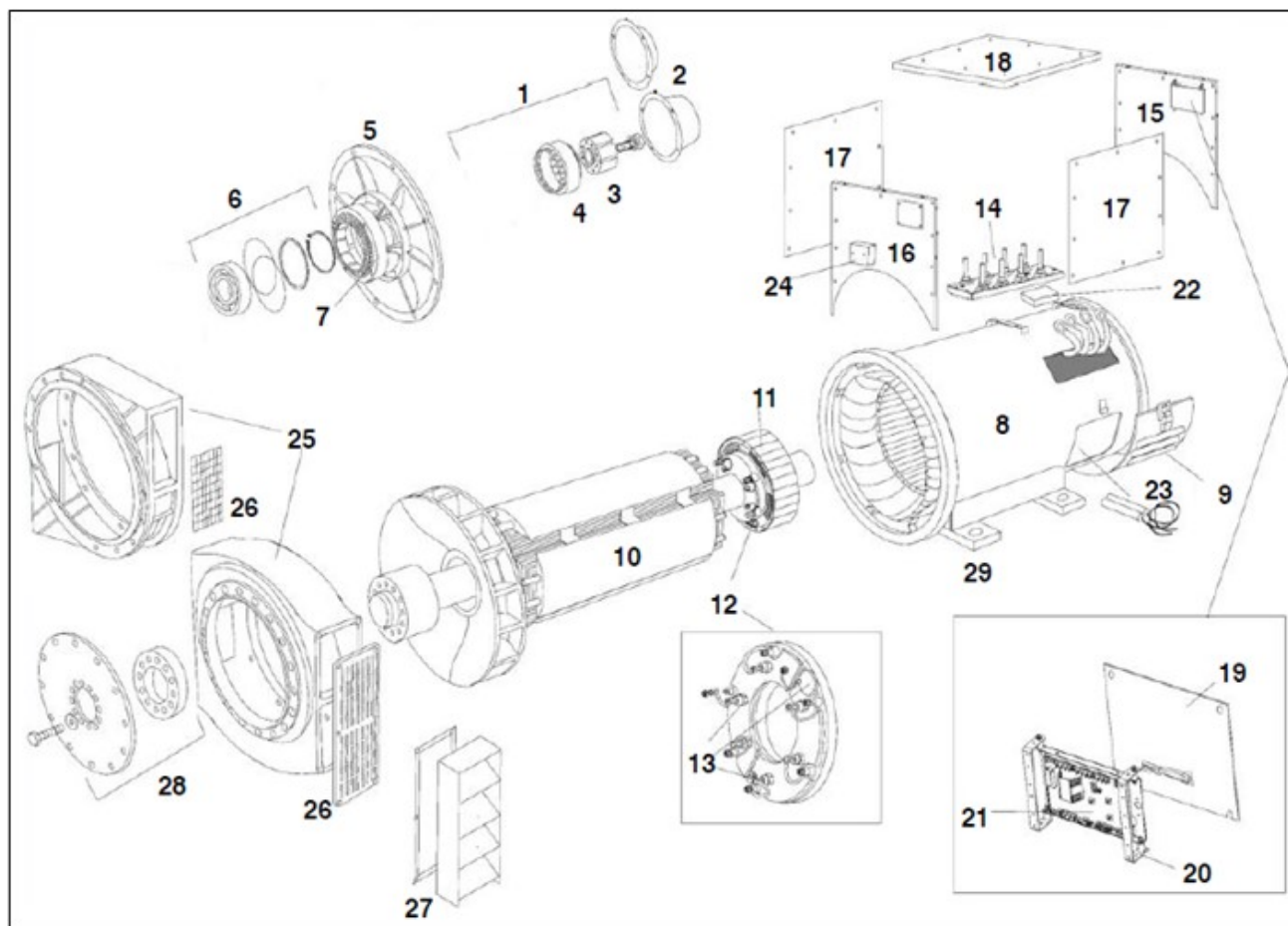
FIGURE 20. S4 (C-F) ONE BEARING ALTERNATOR PARTS DRAWING
