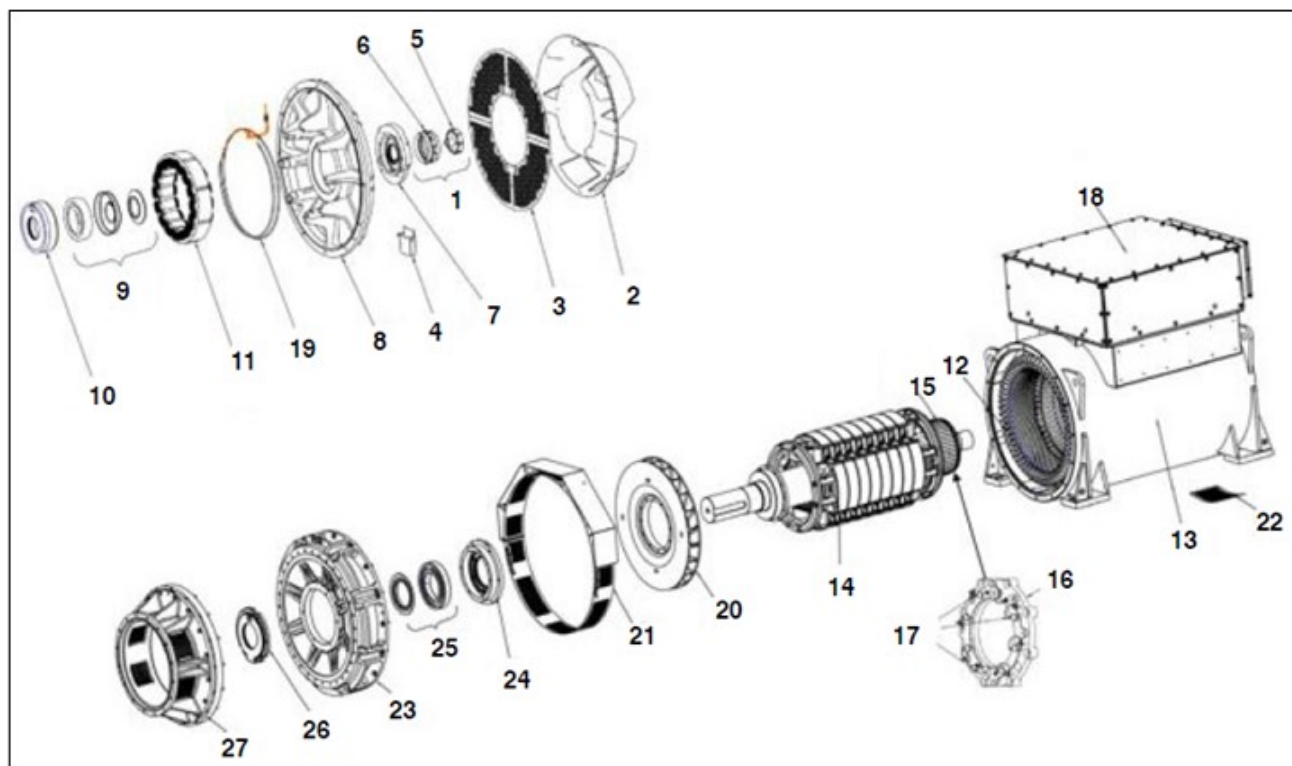
FIGURE 48. S9 HV TWO BEARING ALTERNATOR PARTS DRAWING
