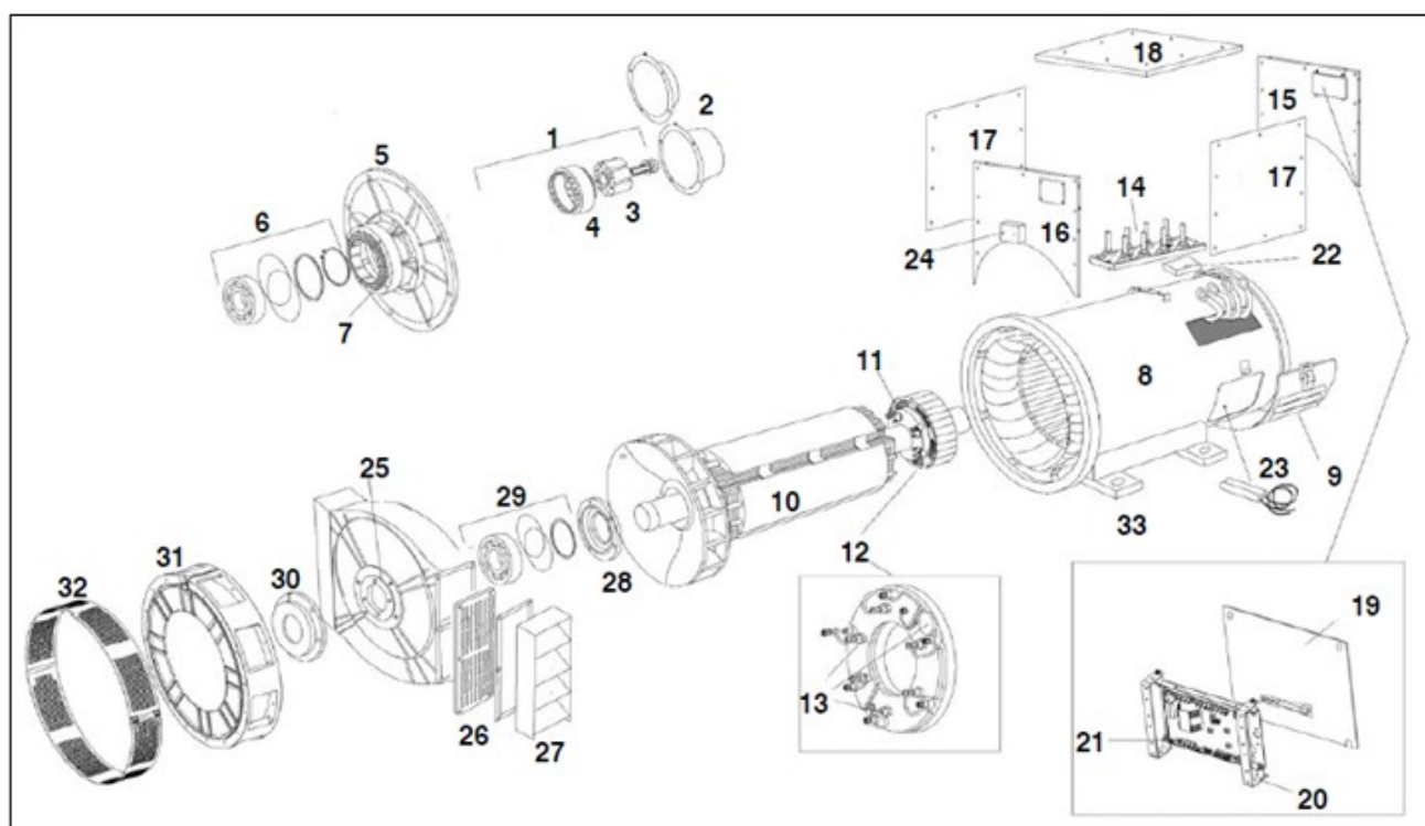
FIGURE 21. S4 (C-F) TWO BEARING ALTERNATOR PARTS DRAWING
