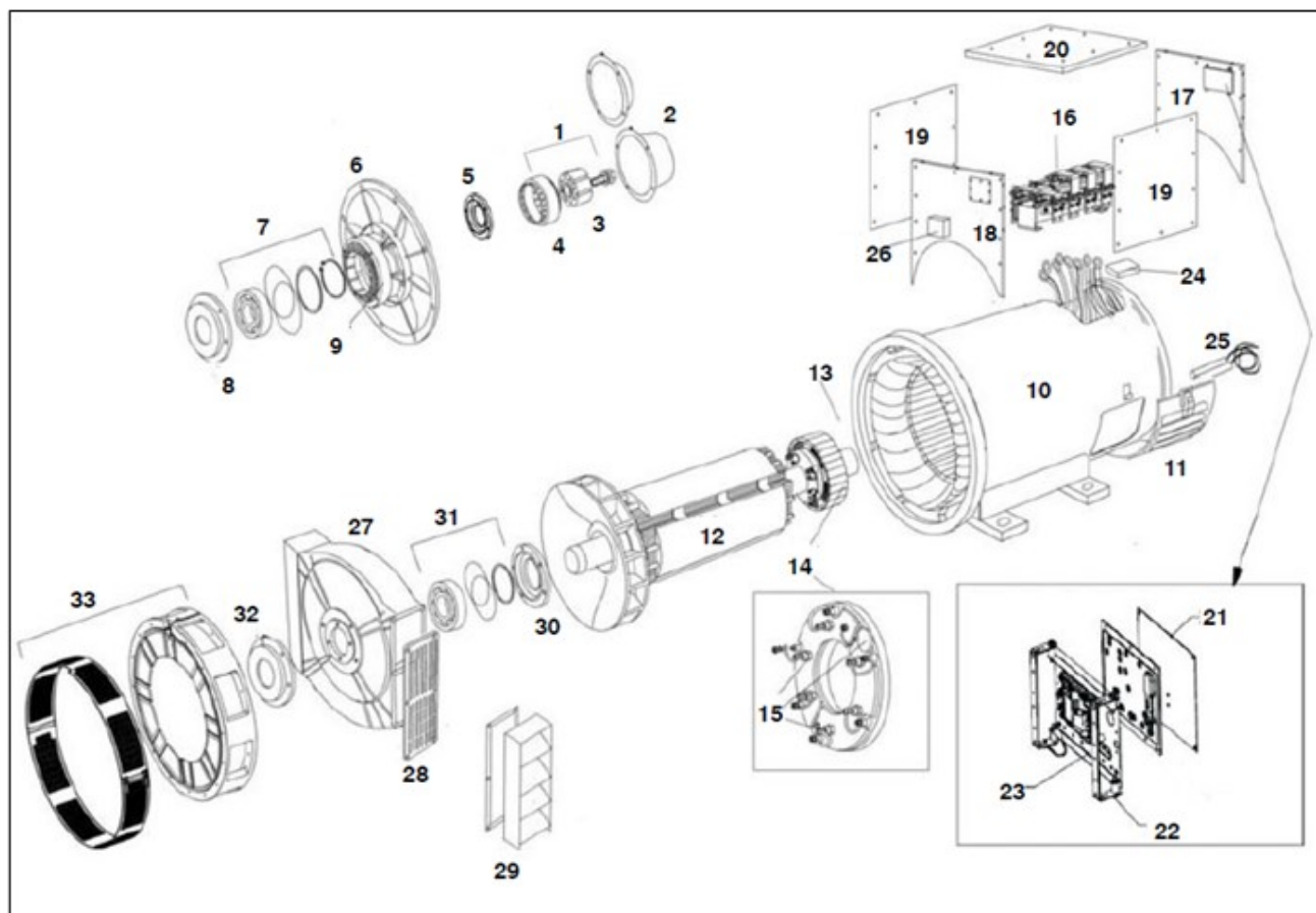
FIGURE 28. S5 (C-F) TWO BEARING ALTERNATOR PARTS DRAWING
