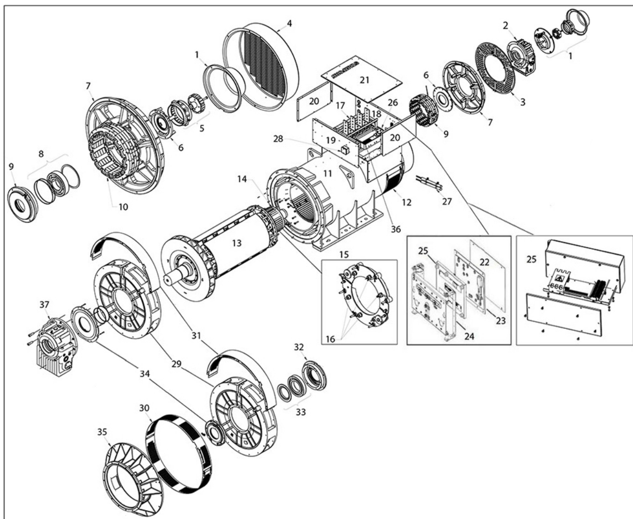
FIGURE 36. S7 LV TWO BEARING ALTERNATOR PARTS DRAWING
