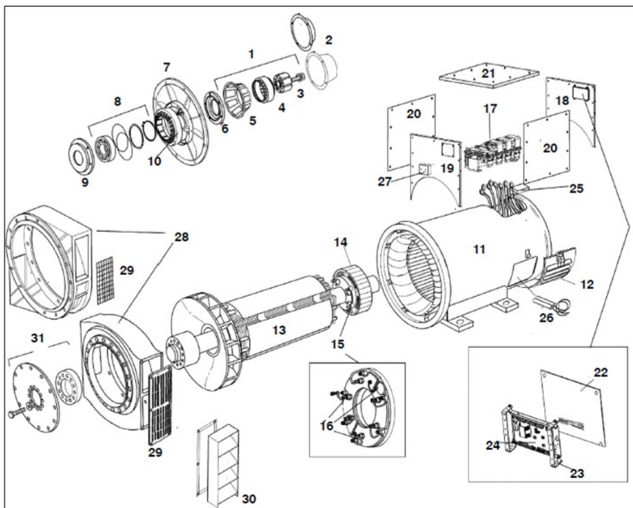
FIGURE 23. HC534 (C-F) ONE BEARING (SER 3-4) ALTERNATOR PARTS DRAWING
