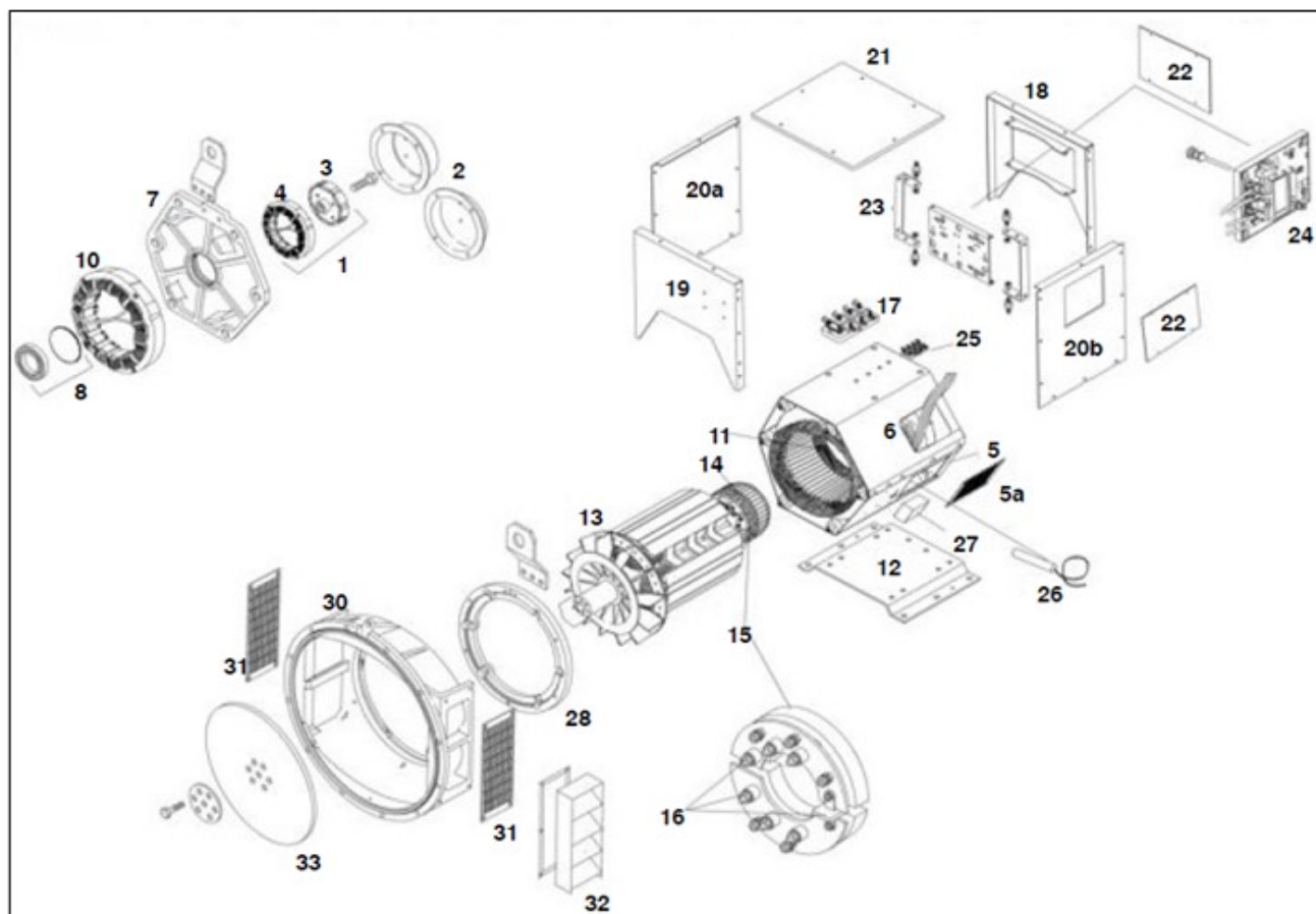
FIGURE 12. UCD22 - ONE BEARING ALTERNATOR PARTS DRAWING
