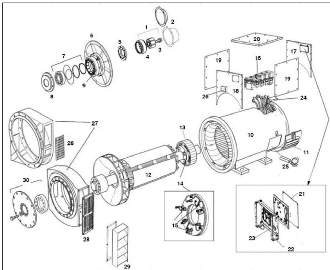
FIGURE 27. S5 (C-F) ONE BEARING ALTERNATOR PARTS DRAWING
