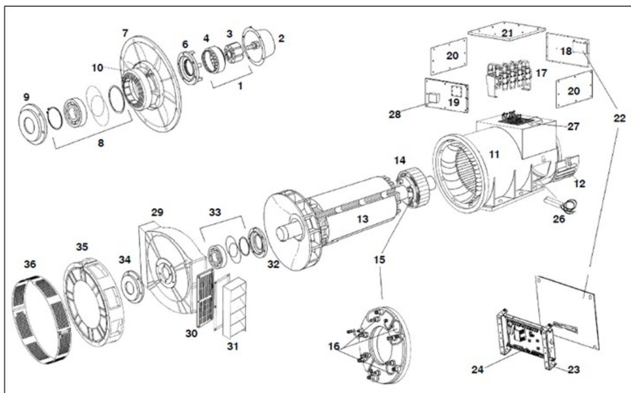
FIGURE 30. HC634 (G-K) TWO BEARING (SER 3) ALTERNATOR PARTS DRAWING
