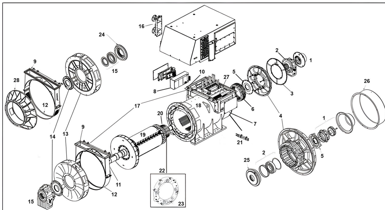
FIGURE 37. S7 WLV TWO BEARING ALTERNATOR PARTS DRAWING
