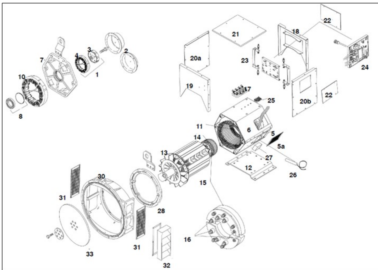
FIGURE 16. UCI274 (C-H) ONE BEARING ALTERNATOR
