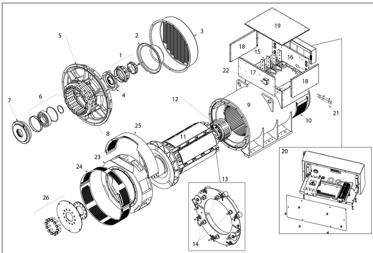
FIGURE 40. A7 LV ONE BEARING ALTERNATOR PARTS DRAWING
