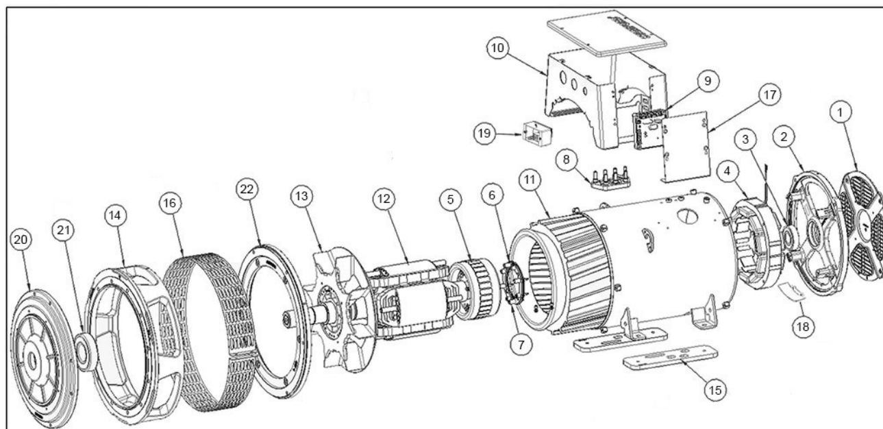
FIGURE 10. S0L2 - TWO BEARING ALTERNATOR PARTS DRAWING
