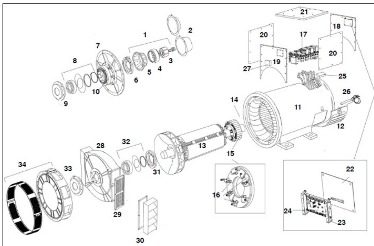
FIGURE 24. HC534 (C-F) TWO BEARING (SER 3-4) ALTERNATOR PARTS DRAWING
