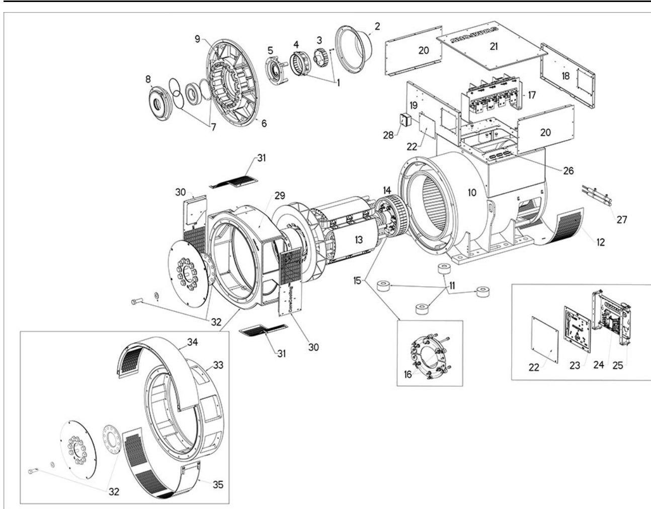
FIGURE 31. S6 (C-H) ONE BEARING (DEDICATED) ALTERNATOR PARTS DRAWING
