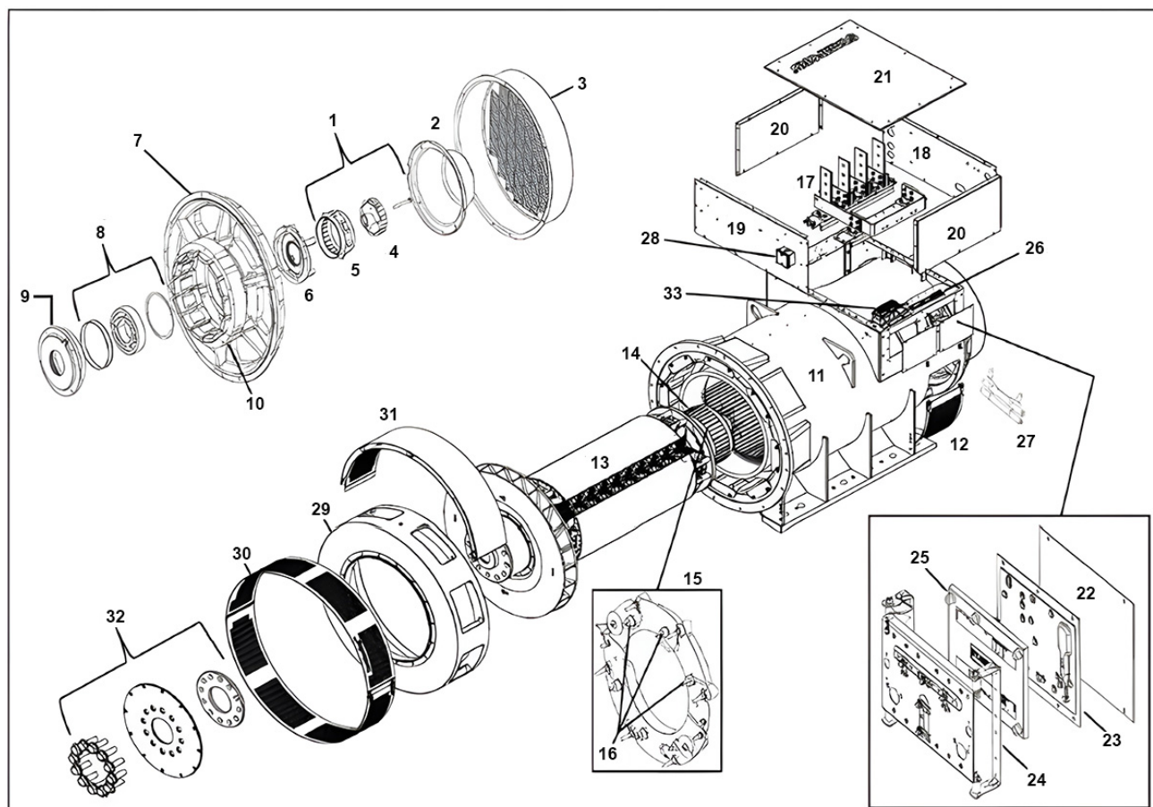
FIGURE 35. S7 LV ONE BEARING ALTERNATOR PARTS DRAWING
