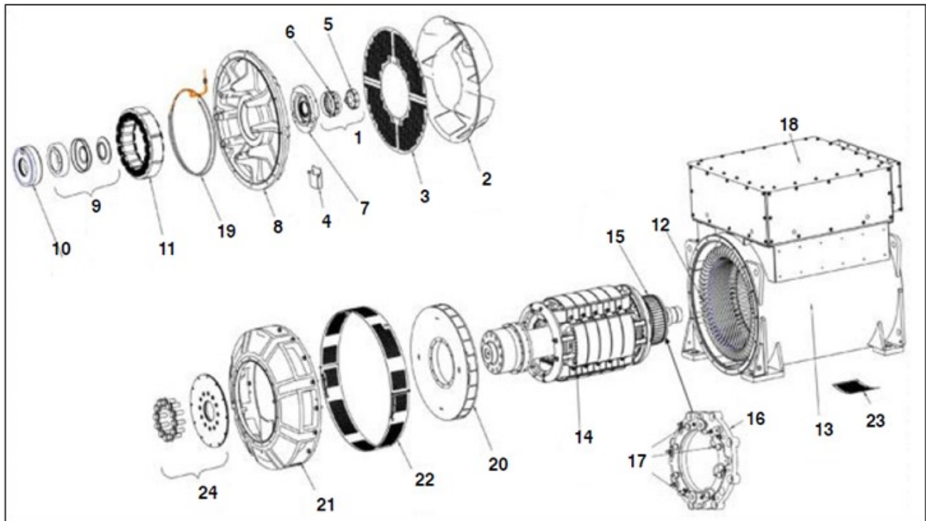
FIGURE 47. S9 HV ONE BEARING ALTERNATOR PARTS DRAWING
