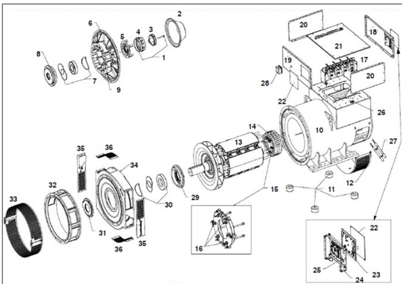
FIGURE 32. S6 (C-H) TWO BEARING (DEDICATED) ALTERNATOR PARTS DRAWING
