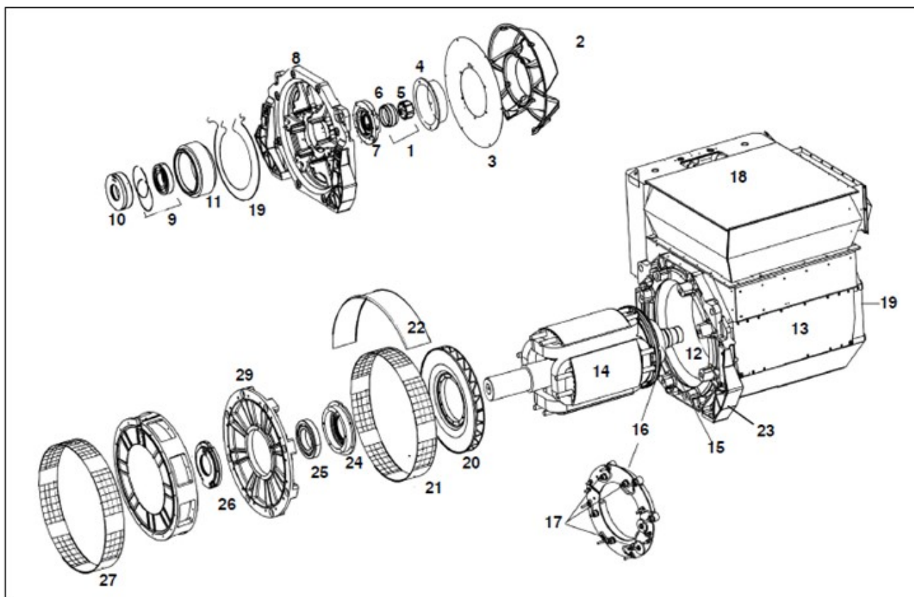
FIGURE 44. P80 TWO BEARING ALTERNATOR PARTS DRAWING
