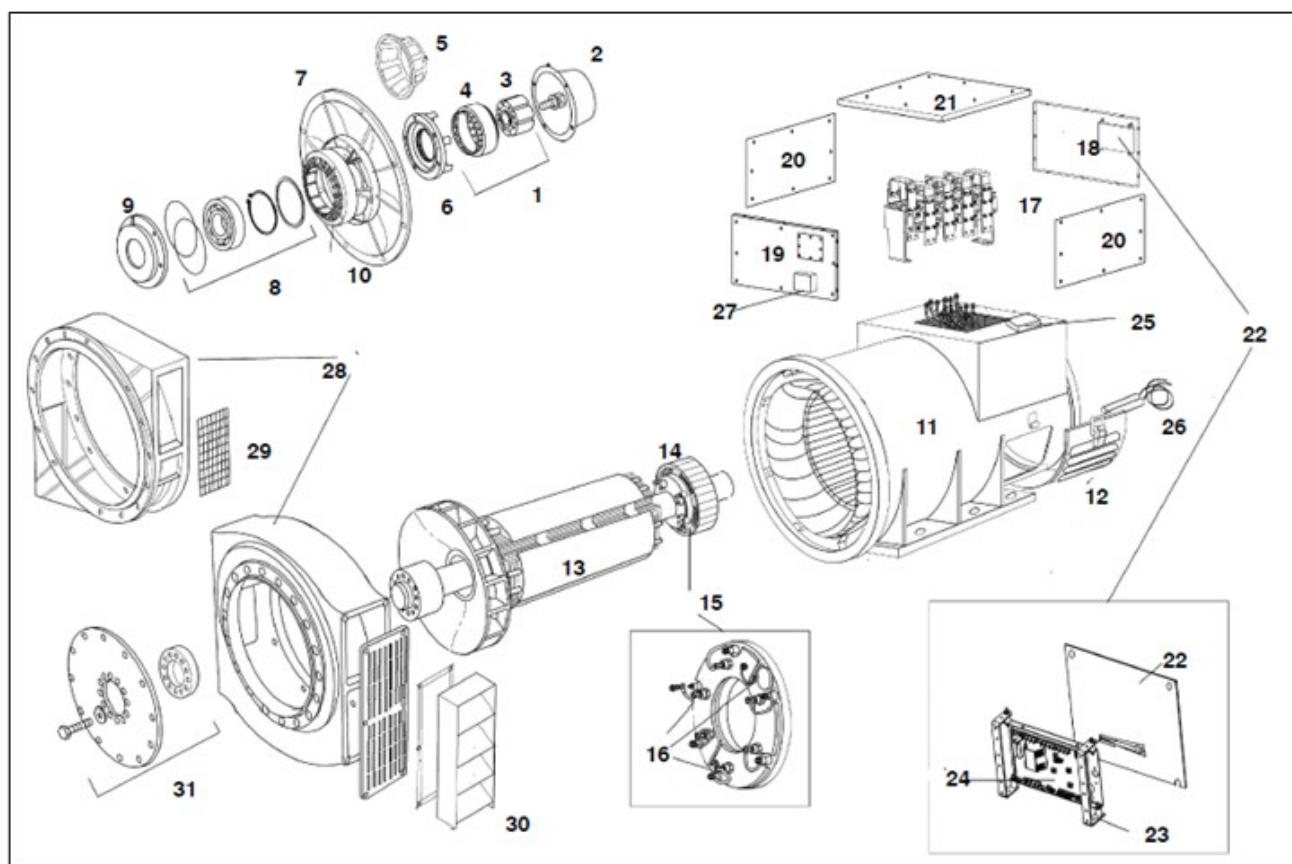
FIGURE 30. HC634 (G-K) ONE BEARING (SER 3) ALTERNATOR PARTS DRAWING
