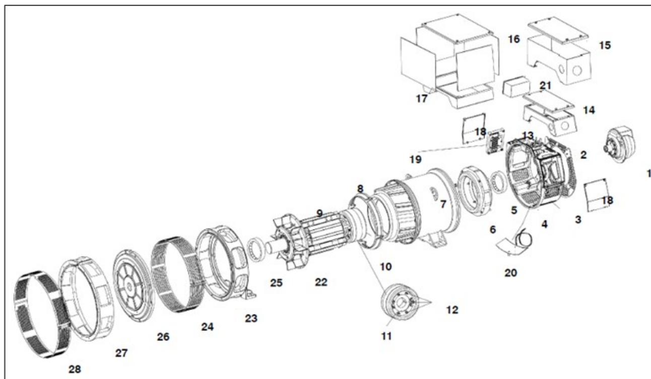
FIGURE 6. P1 - TWO BEARING ALTERNATOR PARTS DRAWING
