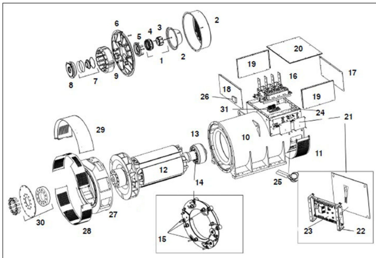
FIGURE 34. P7 (A-G) ONE BEARING ALTERNATOR PARTS DRAWING
