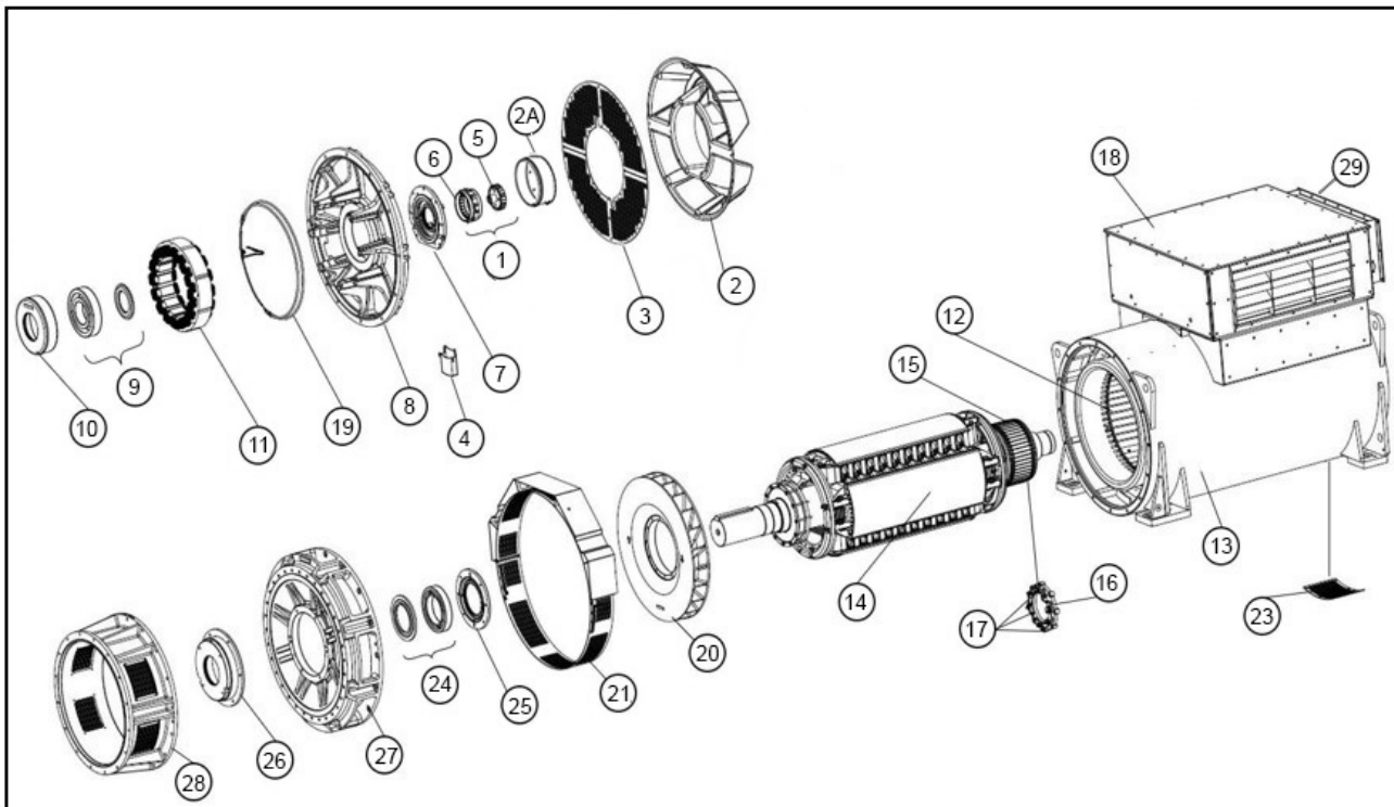
FIGURE 47. S9 LV TWO BEARING ALTERNATOR PARTS DRAWING
