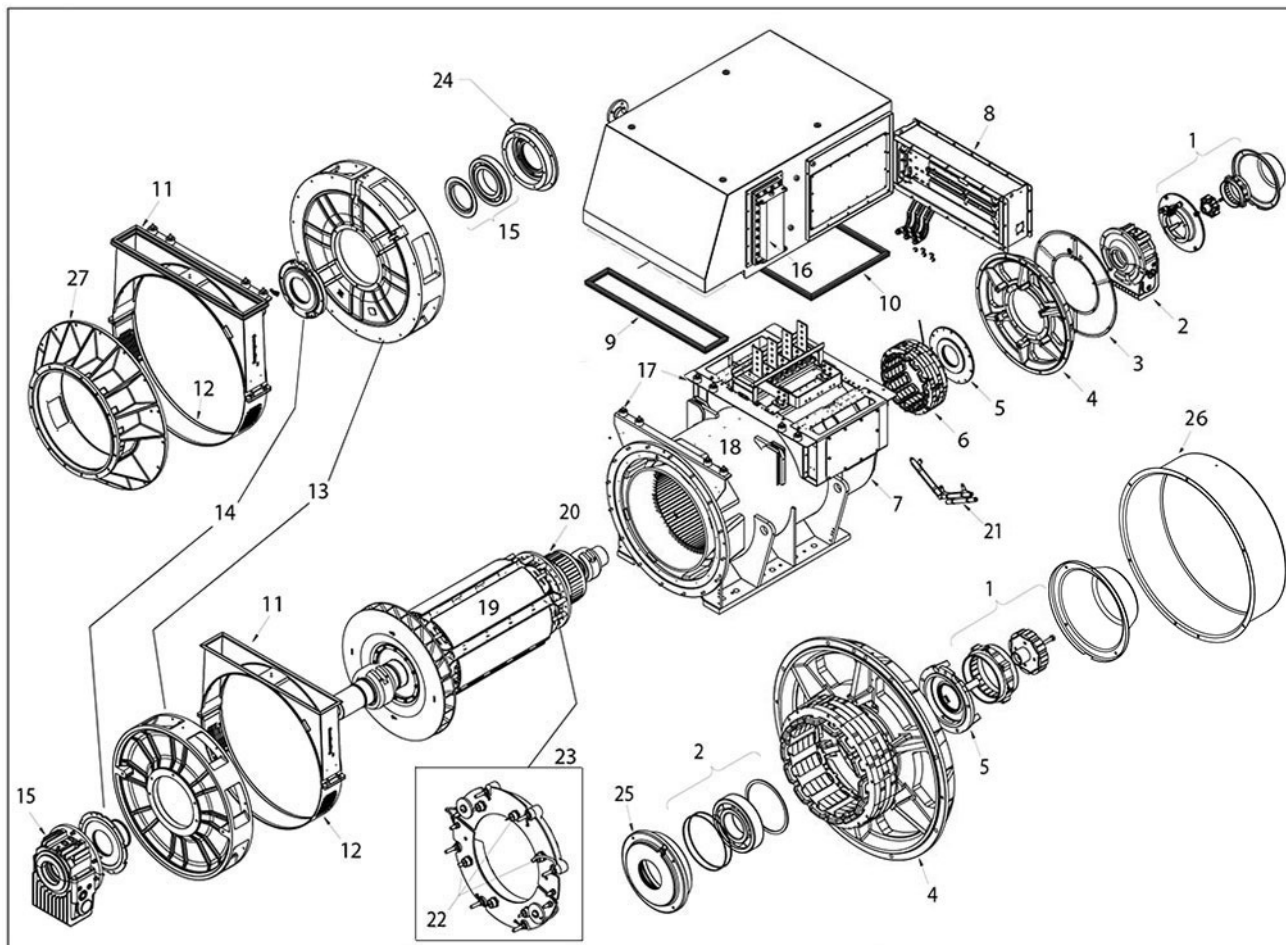
FIGURE 43. A7 WLV TWO BEARING ALTERNATOR PARTS DRAWING
