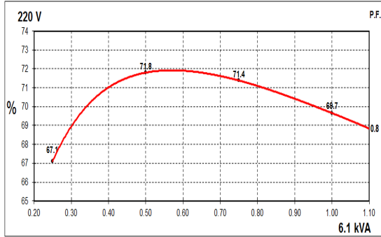
60Hz Curves
