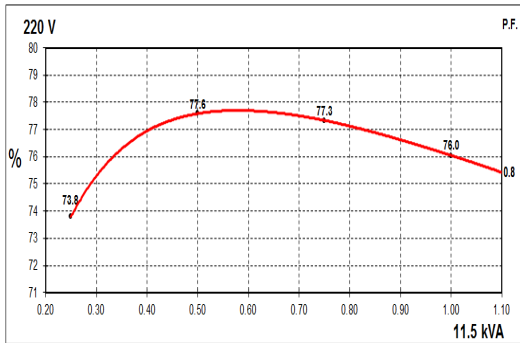
50Hz Curves
