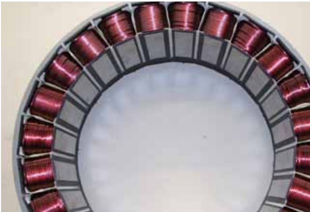
Figure 2: Concentrated non-overlapping wound stator
