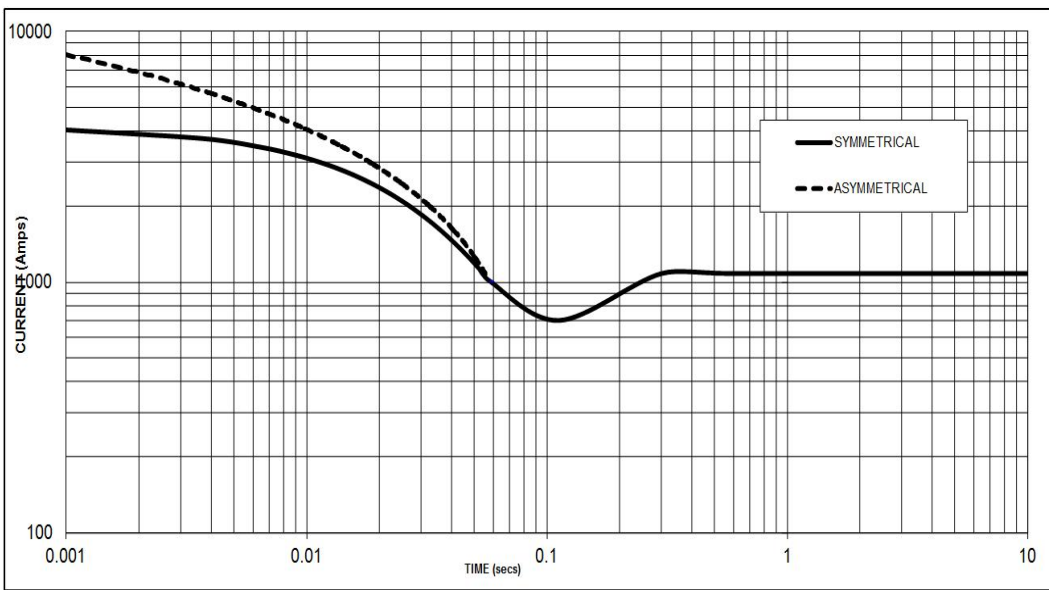
Sustained Short Circuit = 1,080 Amps
