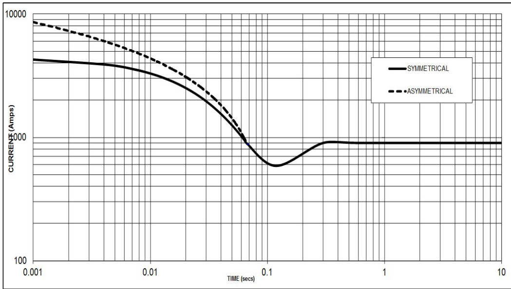
Sustained Short Circuit = 900 Amps
