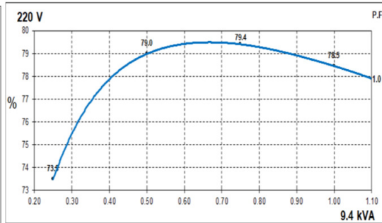
60Hz Curves
