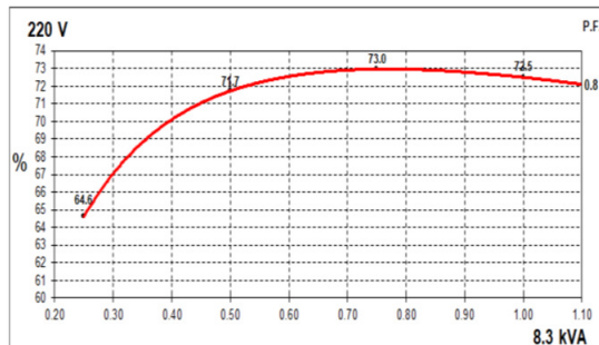
60Hz Curves
