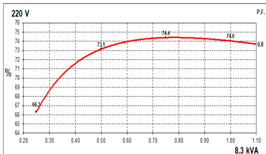
50Hz Curves
