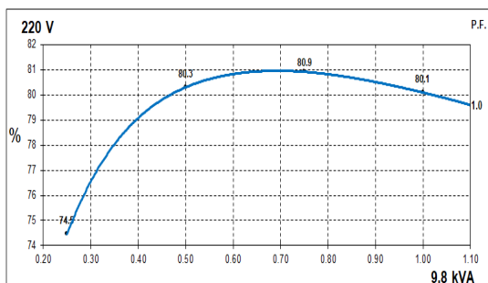
60Hz Curves
