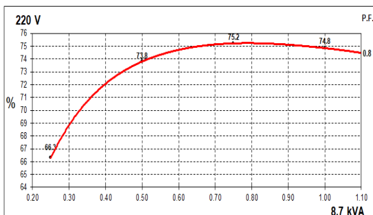
60Hz Curves
