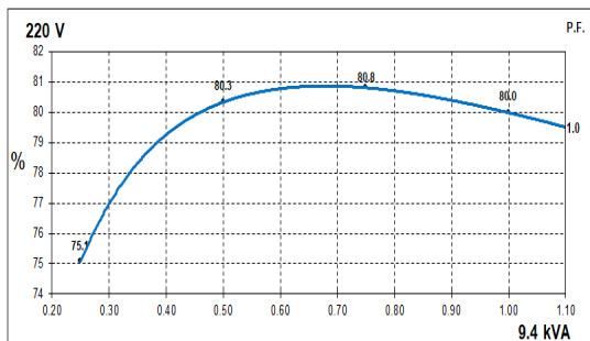
50Hz Curves
