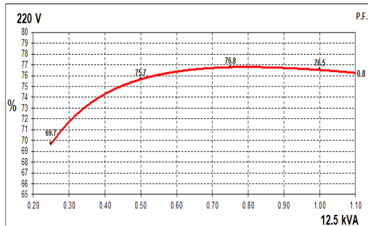
50Hz Curves
