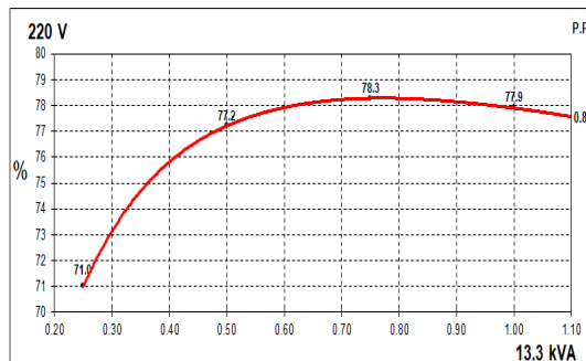
60Hz Curves
