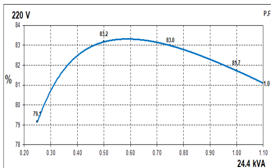
60Hz Curves
