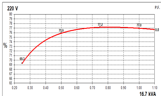
50Hz Curves
