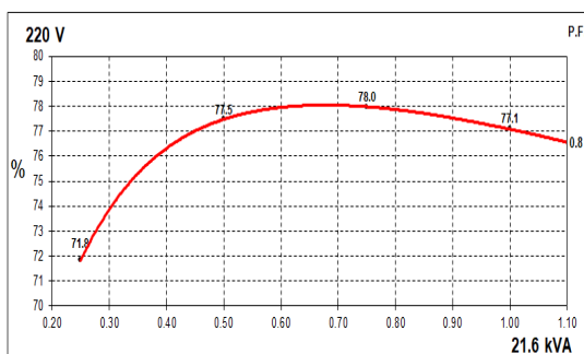
60Hz Curves
