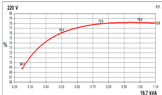
50Hz Curves
