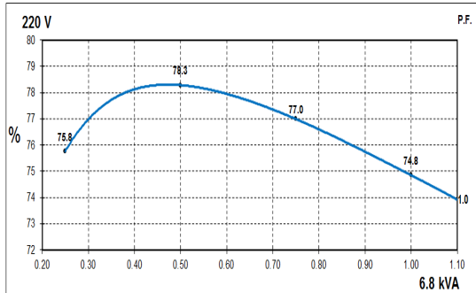
50Hz Curves
