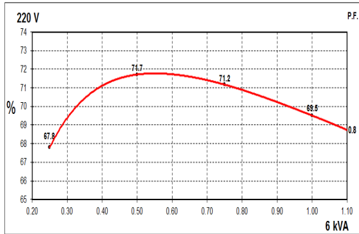
50Hz Curves
