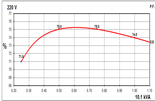
50Hz Curves
