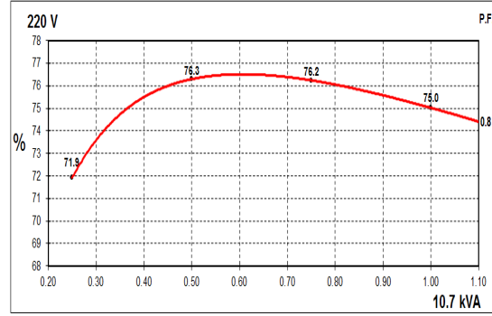
60Hz Curves
