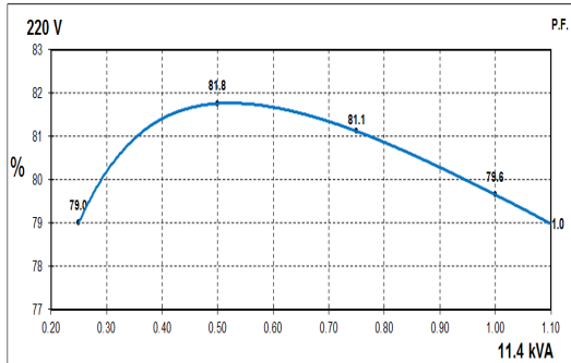
50Hz Curves
