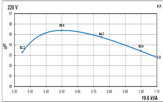
50Hz Curves
