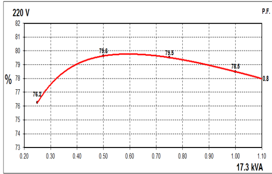
50Hz Curves
