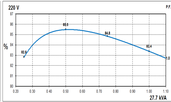
60Hz Curves
