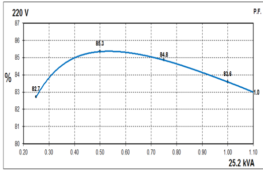
50Hz Curves
