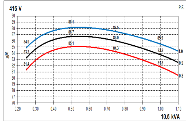
60Hz Curves
