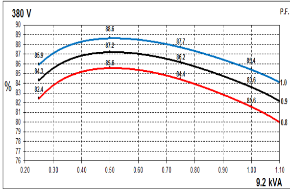
50Hz Curves
