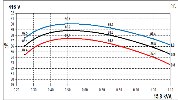
60Hz Curves
