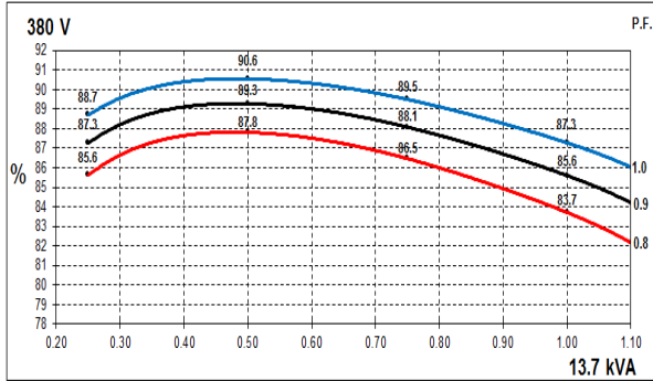
50Hz Curves
