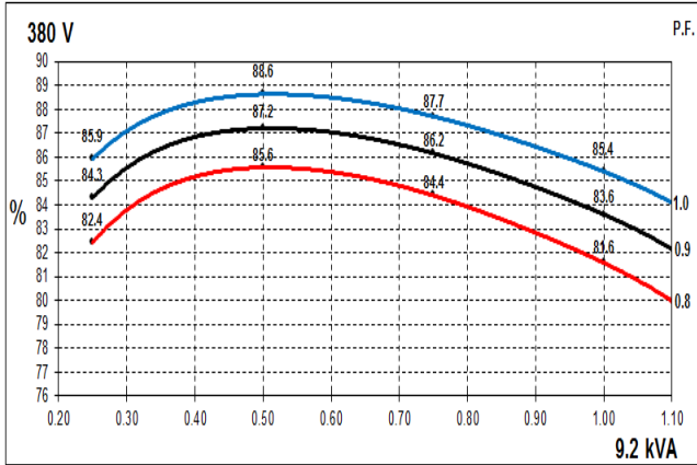
50Hz Curves
