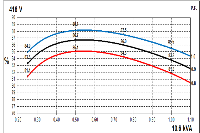
60Hz Curves
