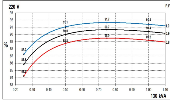
60Hz Curves
