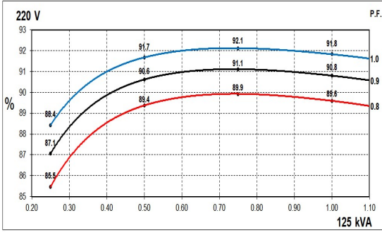
50Hz Curves
