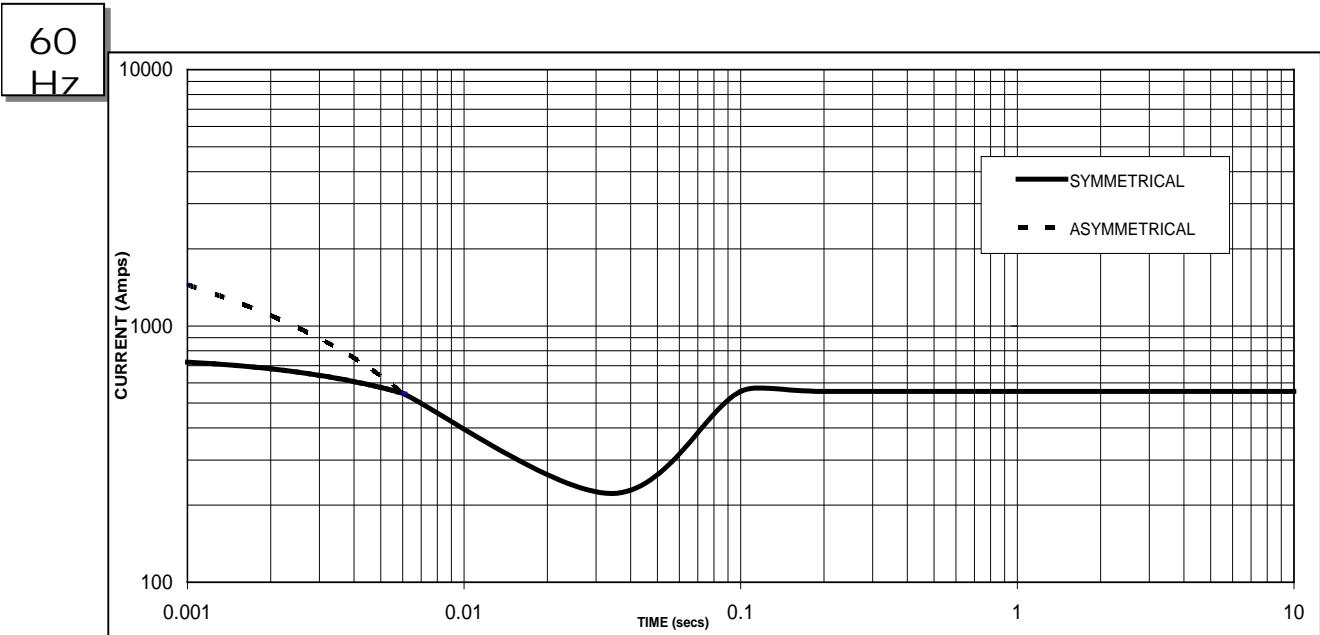
Sustained Short Circuit = 555 Amps
