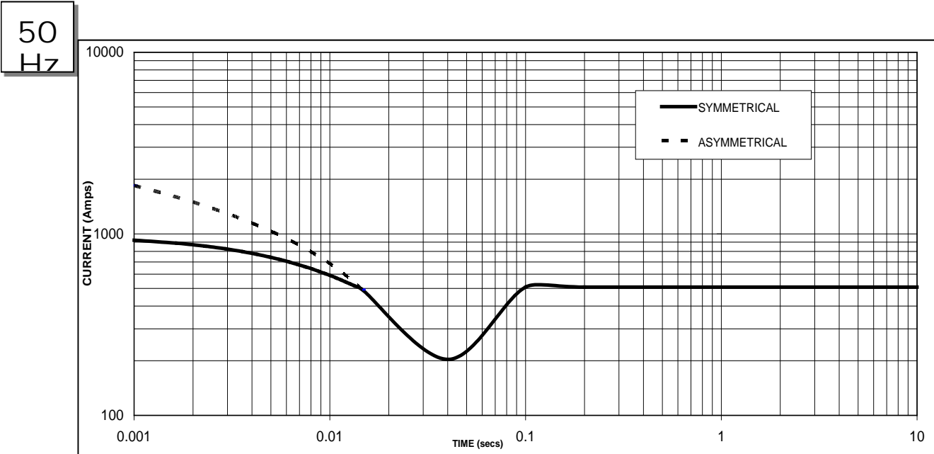
Sustained Short Circuit = 509 Amps
