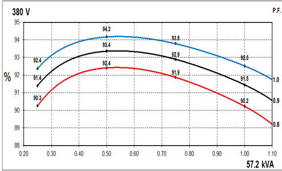
50Hz Curves
