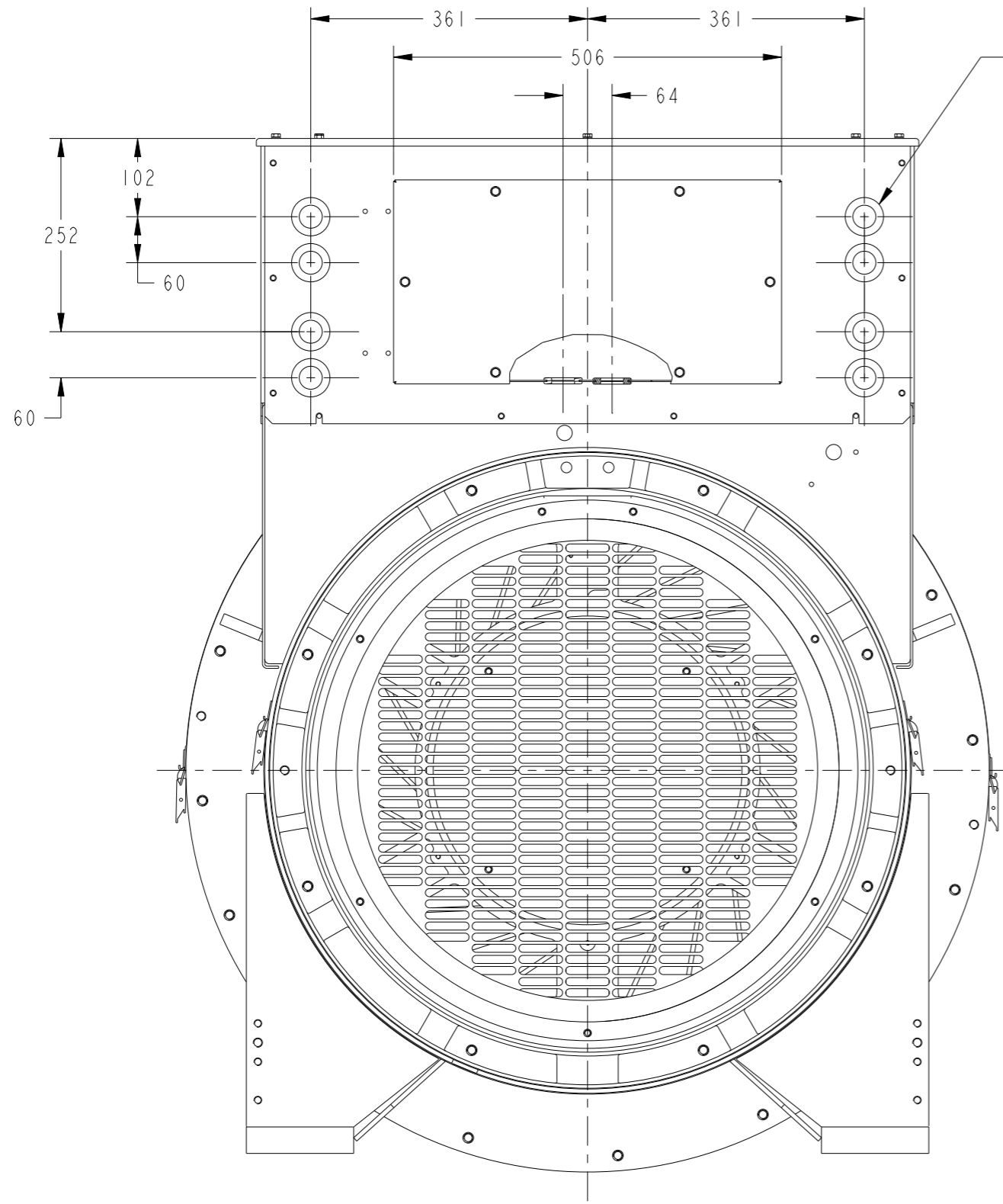
PART SECTION B-B SCALE 1:5
