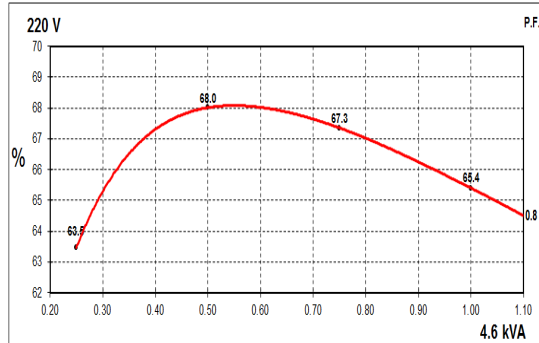
60Hz Curves
