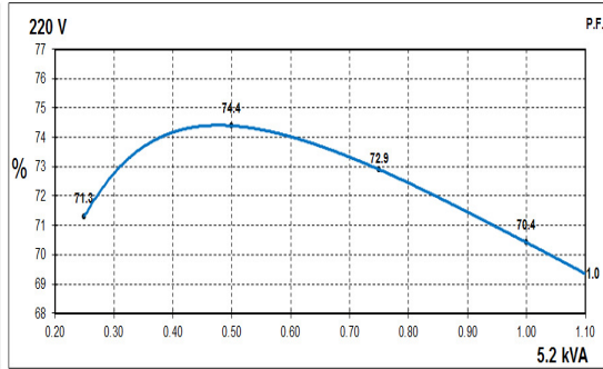
60Hz Curves
