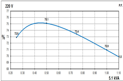
50Hz Curves
