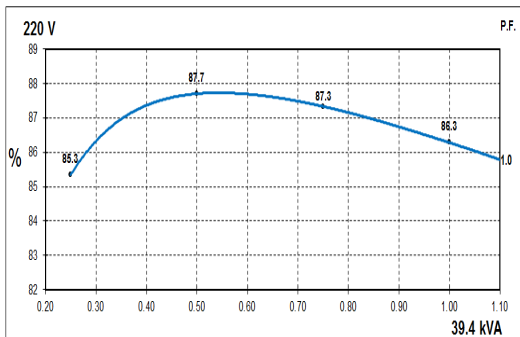
50Hz Curves
