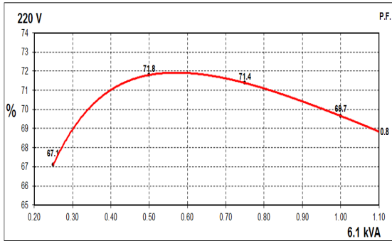
60Hz Curves
