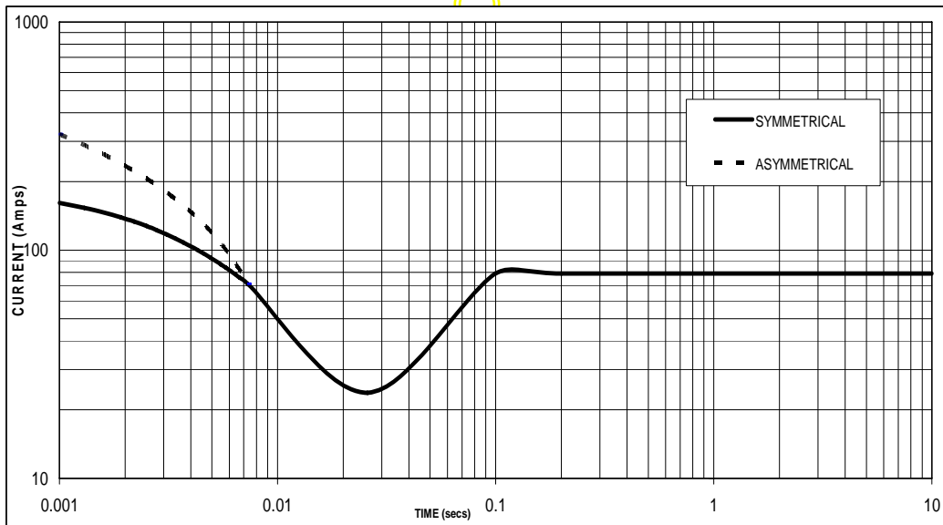
Sustained Short Circuit = 79 Amps
