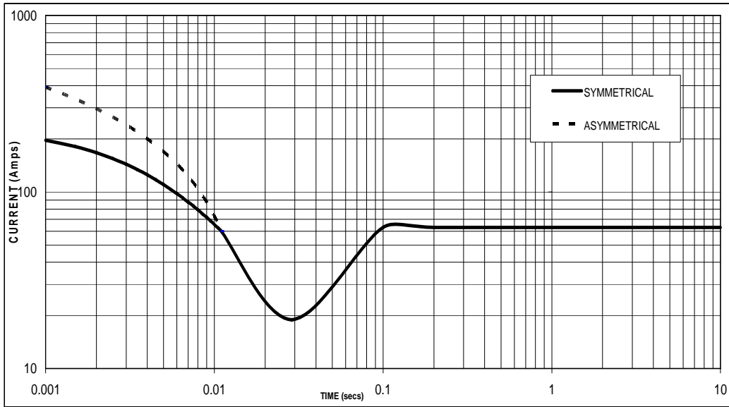
Sustained Short Circuit = 63 Amps
