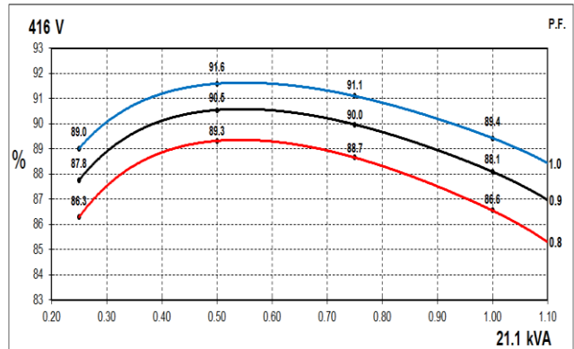
60Hz Curves
