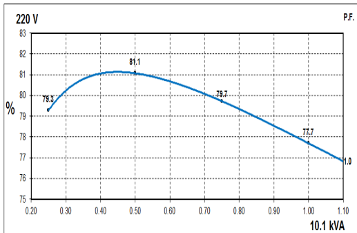
50Hz Curves
