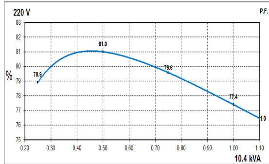
60Hz Curves
