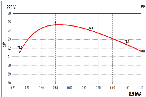
50Hz Curves
