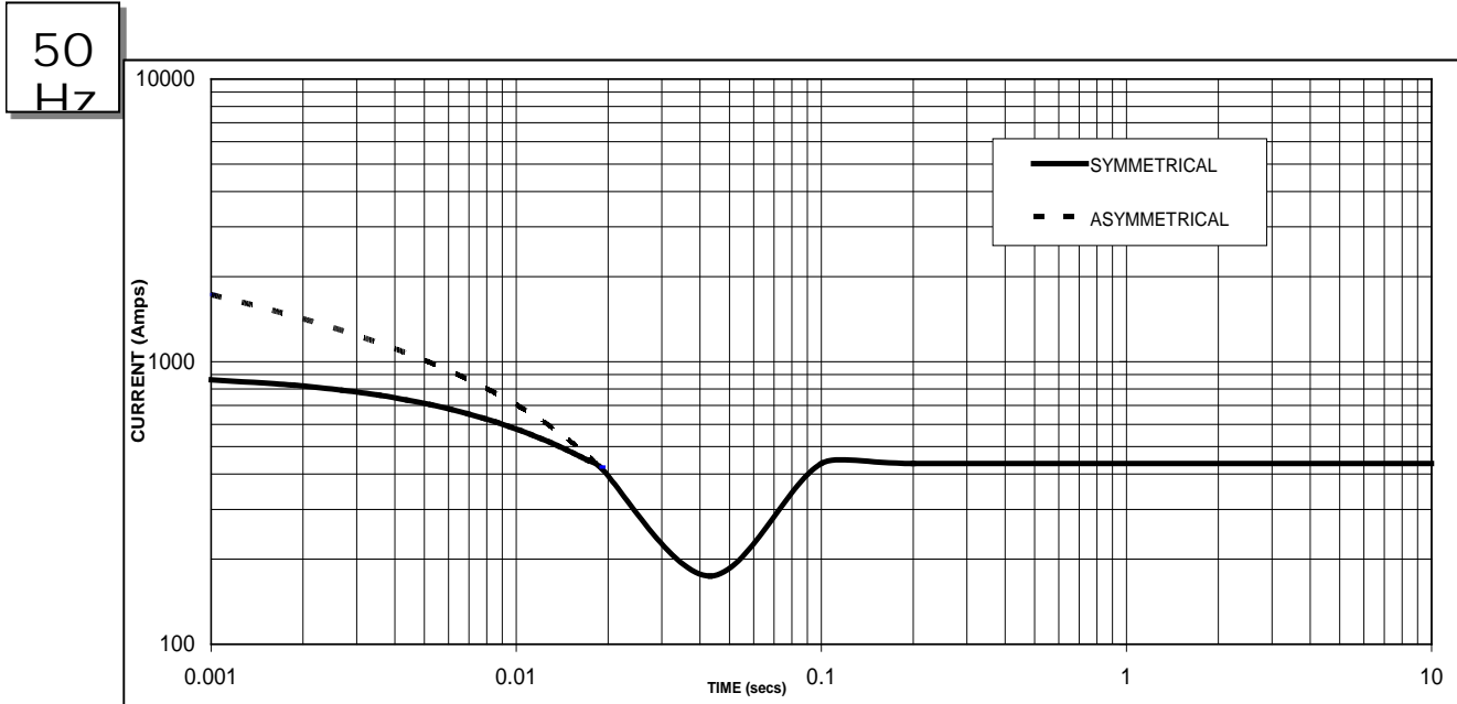
Sustained Short Circuit = 436 Amps
