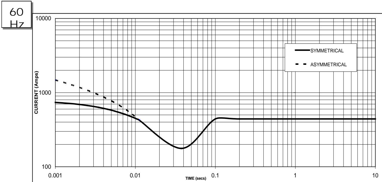
Sustained Short Circuit = 442 Amps
