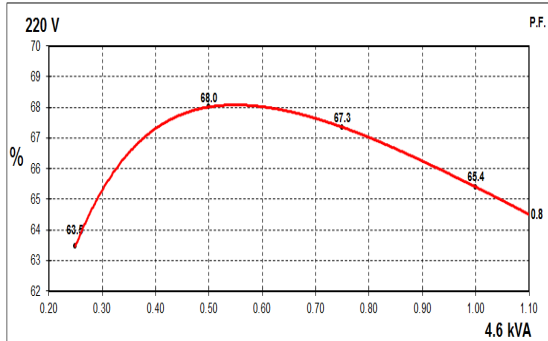
60Hz Curves
