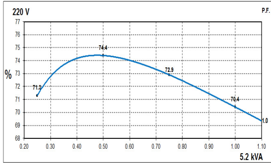
60Hz Curves
