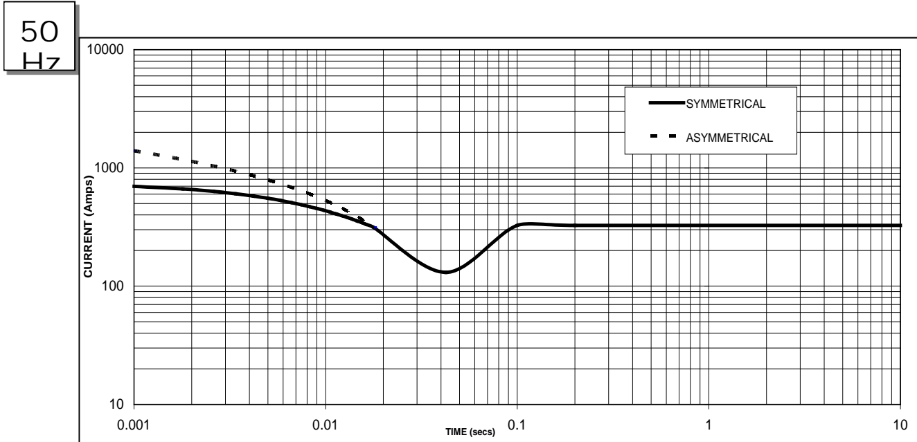
Sustained Short Circuit = 327 Amps
