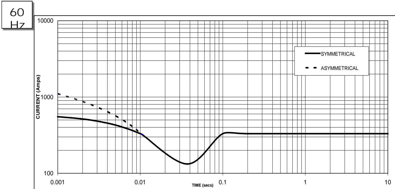
Sustained Short Circuit = 331 Amps
